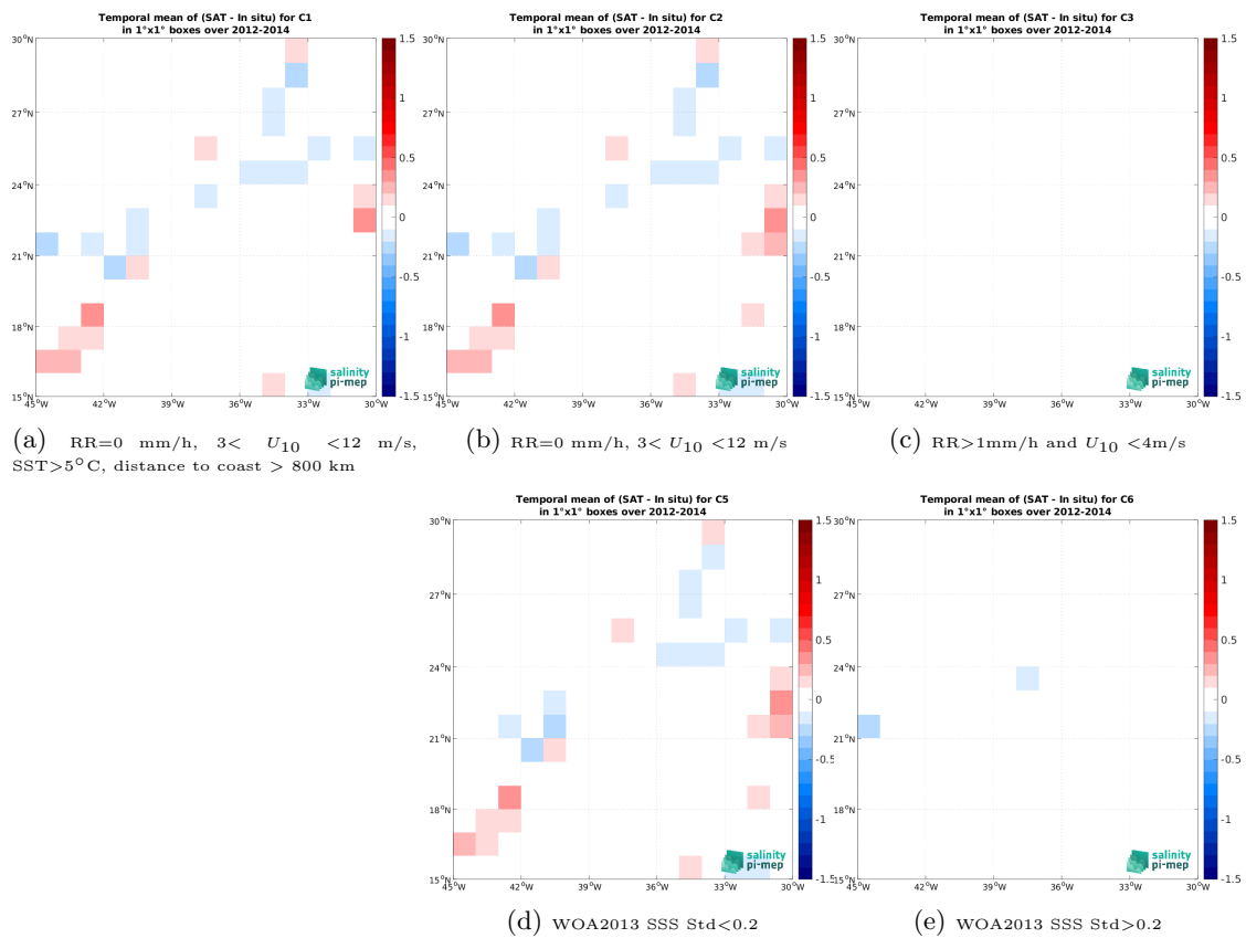
Figure 14: Temporal mean gridded over spatial boxes of size 1^\circ \times 1^\circ of \Delta\text{SSS} (Aquarius SSS L4 OI v5 - Weekly (IPRC) - TSG (GOSUD-Research-vessel)) for 5 different subdatasets corresponding to:RR=0 mm/h, 3 < U_{10} < 12 m/s, SST>5°C, distance to coast > 800 km (a), RR=0 mm/h, 3 < U_{10} < 12 m/s (b), RR>1mm/h and U_{10} < 4 m/s (c), WOA2013 SSS Std<0.2 (d), WOA2013 SSS Std>0.2 (e).
