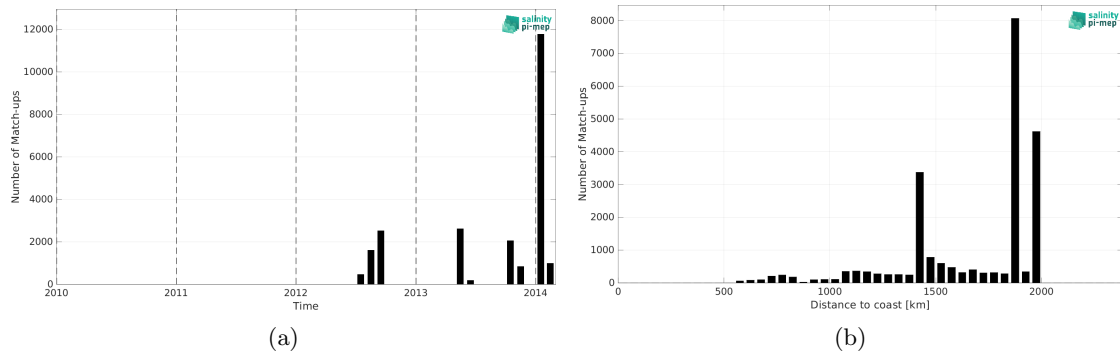
Figure 2: Number of match-ups between TSG (GOSUD-Research-vessel) and Aquarius SSS L4 OI v5 - Weekly (IPRC) SSS as a function of time (a) and as function of the distance to coast (b) over the SPURS 1 Pi-MEP region and for the full satellite product period.
