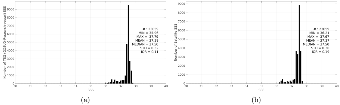
Figure 3: Histograms of SSS from TSG (GOSUD-Research-vessel) (a) and Aquarius SSS L4 OI v5 - Weekly (IPRC) (b) considering all match-up pairs per bins of 0.1 over the SPURS 1 Pi-MEP region and for the full satellite product period.
