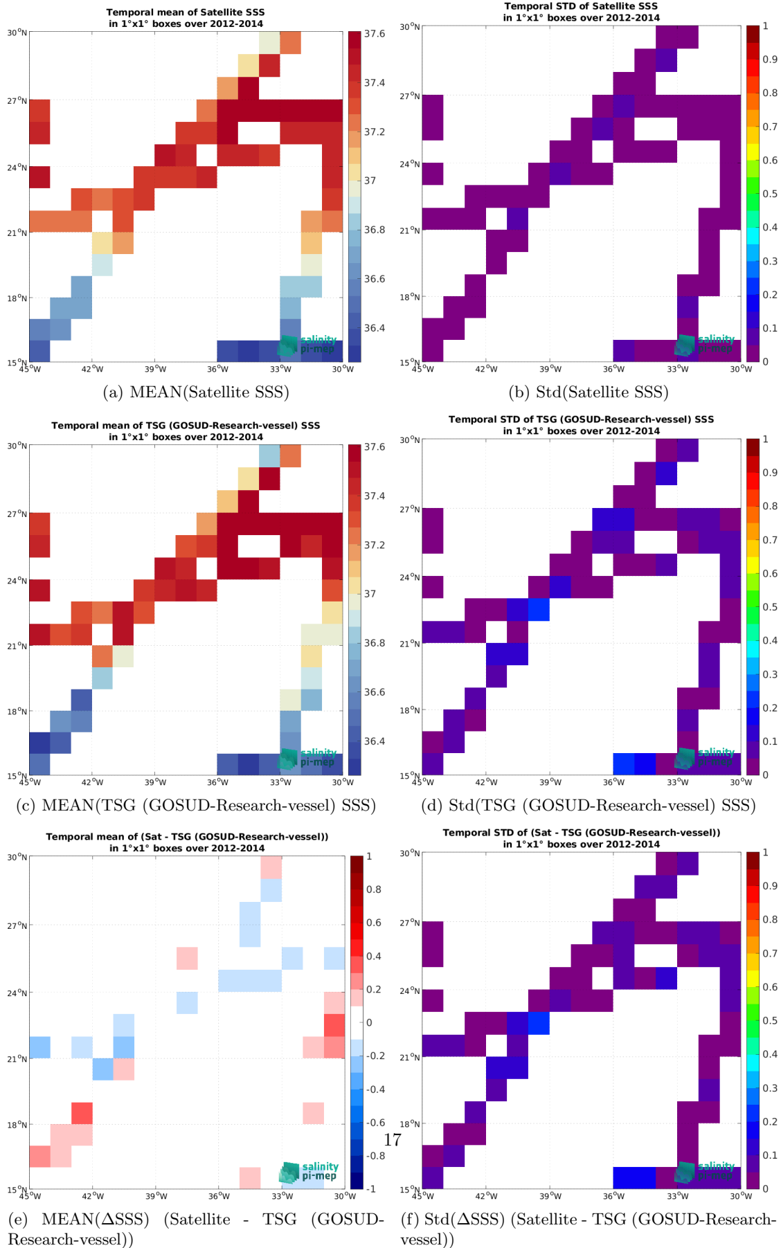
Figure 7: Temporal mean (left) and Std (right) of SSS from Aquarius SSS L4 OI v5 - Weekly (IPRC) (top), TSG (GOSUD-Research-vessel) (middle), and of \Delta SSS (Satellite - TSG (GOSUD-Research-vessel)). Only match-up pairs are used to generate these maps.
