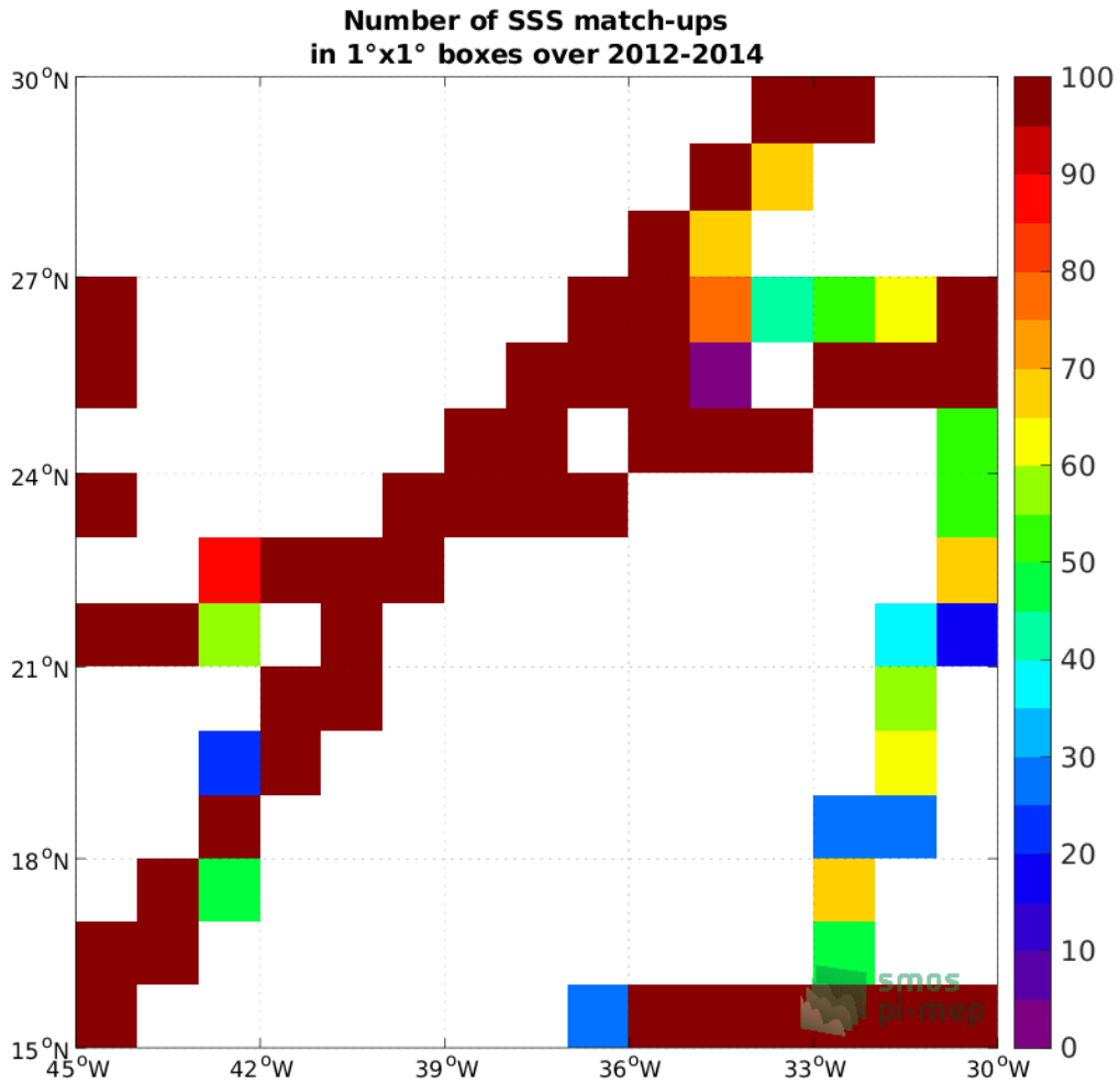
Figure 4: Number of SSS match-ups between TSG (GOSUD-Research-vessel) SSS and the Aquarius SSS L4 OI v5 - Weekly (IPRC) SSS product for the SPURS 1 Pi-MEP region over 1^\circ \times 1^\circ boxes and for the full satellite product period.
