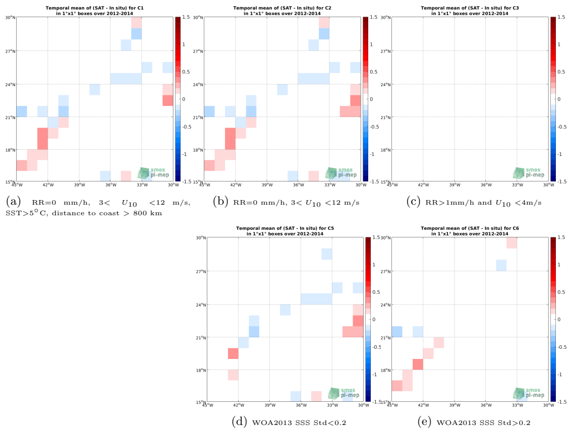
Figure 12: Temporal mean gridded over spatial boxes of size 1°x1° of \Delta SSS (Aquarius SSS L4 OI v5 - Weekly (IPRC) - TSG (GOSUD-Research-vessel)) for 5 different subdatasets corresponding to:RR=0 mm/h, 3 < U_{10} < 12 m/s, SST>5°C, distance to coast > 800 km (a), RR=0 mm/h, 3 < U_{10} < 12 m/s (b), RR>1mm/h and U_{10} < 4 m/s (c), WOA2013 SSS Std<0.2 (d), WOA2013 SSS Std>0.2 (e).
