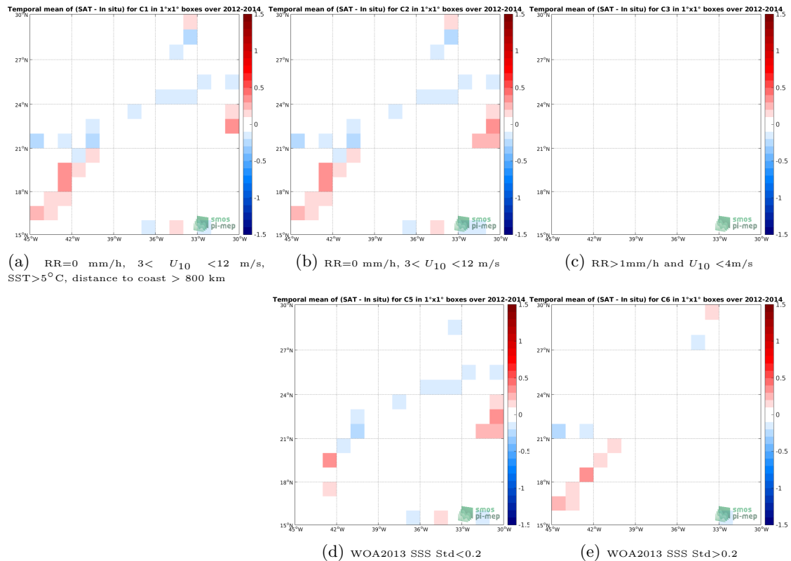
Figure 12: Temporal mean gridded over spatial boxes of size 1^\circ \times 1^\circ of \Delta SSS (Aquarius-L4-IPRC-V5-WEEKLY - TSG-GOSUD-Research-vessel) for 5 different subdatasets corresponding to:RR=0 mm/h, 3 < U_{10} < 12 m/s, SST >5^\circ C, distance to coast > 800 km (a), RR=0 mm/h, 3 < U_{10} < 12 m/s (b), RR >1 mm/h and U_{10} < 4 m/s (c), WOA2013 SSS Std <0.2 (d), WOA2013 SSS Std >0.2 (e).
