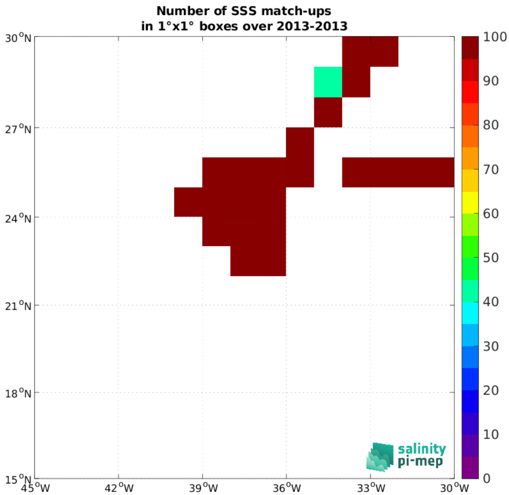
Figure 5: Number of SSS match-ups between TSG (CSIC-UTM) SSS and the Aquarius SSS L4 OI v5 - Weekly (IPRC) SSS product for the SPURS 1 Pi-MEP region over 1^\circ \times 1^\circ boxes and for the full satellite product period.
