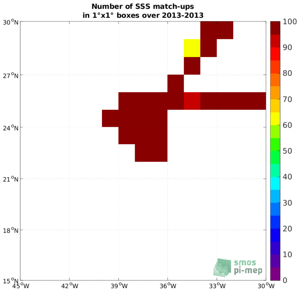
Figure 4: Number of SSS match-ups between TSG (CSIC-UTM) SSS and the Aquarius SSS L4 OI v5 - Weekly (IPRC) SSS product for the SPURS 1 Pi-MEP region over 1°×1° boxes and for the full satellite product period.
