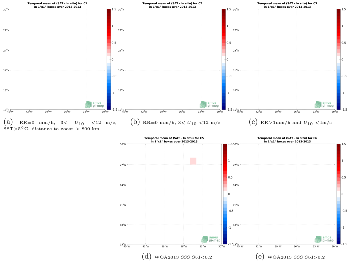
Figure 12: Temporal mean gridded over spatial boxes of size 1^{\circ}\times 1^{\circ} of \Delta\text{SSS} (Aquarius SSS L4 OI v5 - Weekly (IPRC) - TSG (CSIC-UTM)) for 5 different subdatasets corresponding to:RR=0 mm/h, 3 < U_{10} < 12 m/s, SST >5^{\circ}\text{C} , distance to coast > 800 km (a), RR=0 mm/h, 3 < U_{10} < 12 m/s (b), RR >1 mm/h and U_{10} < 4 m/s (c), WOA2013 SSS Std <0.2 (d), WOA2013 SSS Std >0.2 (e).
