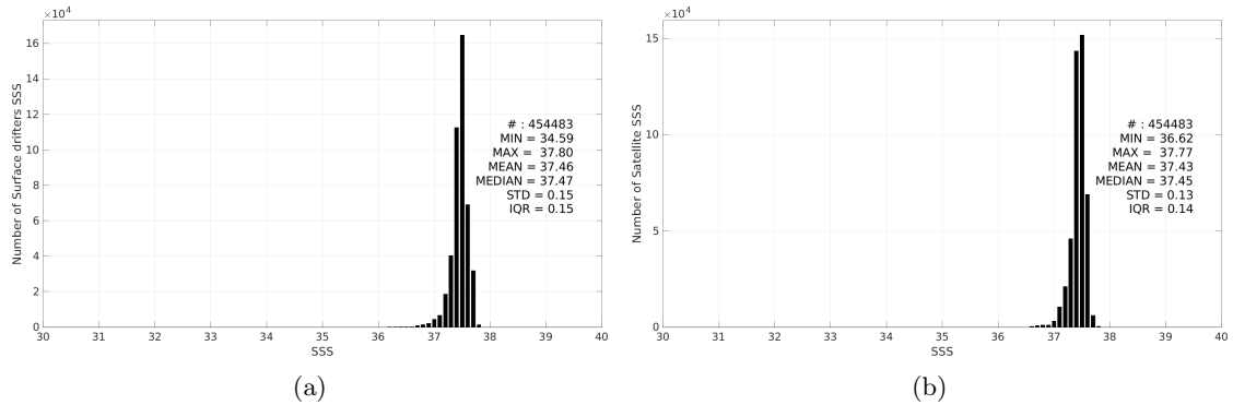
Figure 3: Histograms of SSS from Surface drifters (a) and Aquarius SSS L4 OI v5 - Weekly (IPRC) (b) considering all match-up pairs per bins of 0.1 over the SPURS 1 Pi-MEP region and for the full satellite product period.
