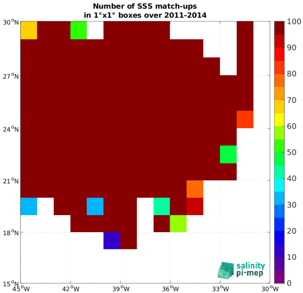
Figure 3: Number of SSS match-ups between Surface drifters SSS and the Aquarius SSS L4 OI v5 - Weekly (IPRC) SSS product for the SPURS 1 Pi-MEP region over 1^\circ \times 1^\circ boxes and for the full satellite product period.
