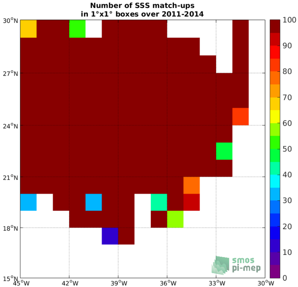
Figure 3: Number of SSS match-ups between Surface drifters SSS and the Aquarius-L4-IPRC-V5-WEEKLY SSS product for the SPURS 1 Pi-MEP region over 1°x1° boxes and for the full satellite product period.
