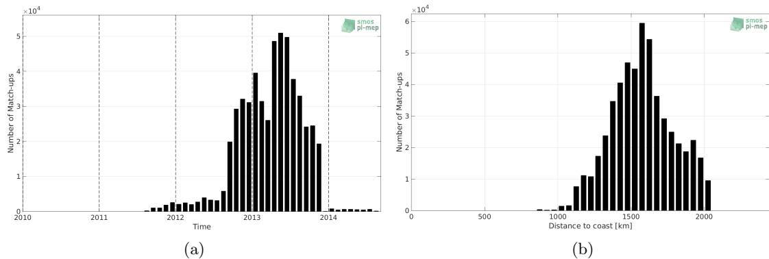
Figure 1: Number of match-ups between Surface drifters and Aquarius-L4-IPRC-V5-WEEKLY SSS as a function of time (a) and as function of the distance to coast (b) over the SPURS 1 Pi-MEP region and for the full satellite product period.
