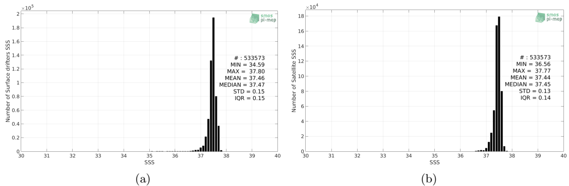
Figure 2: Histograms of SSS from Surface drifters (a) and Aquarius-L4-IPRC-V5-WEEKLY (b) considering all match-up pairs per bins of 0.1 over the SPURS 1 Pi-MEP region and for the full satellite product period.
