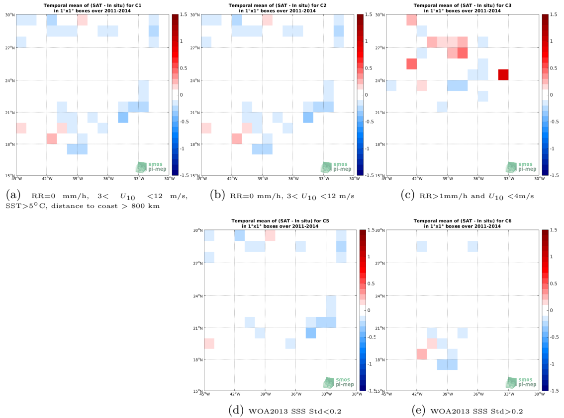
Figure 11: Temporal mean gridded over spatial boxes of size 1^\circ \times 1^\circ of \Delta SSS (Aquarius-L4-IPRC-V5-WEEKLY - Surface drifters) for 5 different subdatasets corresponding to:RR=0 mm/h, 3 < U_{10} < 12 m/s, SST >5^\circ C, distance to coast > 800 km (a), RR=0 mm/h, 3 < U_{10} < 12 m/s (b), RR >1 mm/h and U_{10} < 4 m/s (c), WOA2013 SSS Std <0.2 (d), WOA2013 SSS Std >0.2 (e).
