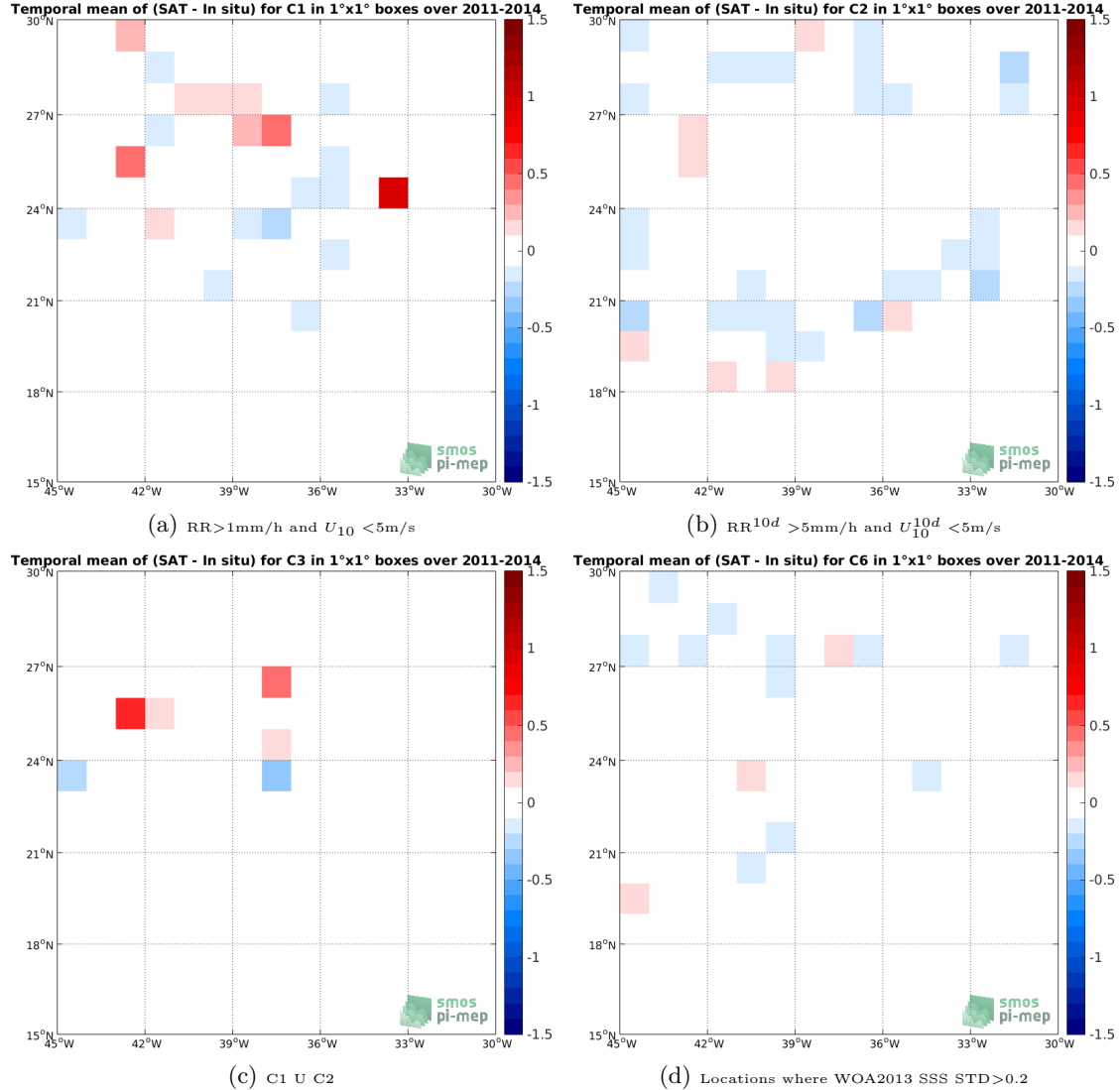
Figure 11: Temporal mean gridded over spatial boxes of size 1^\circ \times 1^\circ of \Delta SSS (Aquarius-L4-IPRC-V5-WEEKLY - Surface drifters) for 4 different subdatasets corresponding to: RR > 1\text{mm/h} and U_{10} < 5\text{m/s} (a), RR^{10d} > 5\text{mm/h} and U_{10}^{10d} < 5\text{m/s} (b), C1 U C2 (c), Locations where WOA2013 SSS STD > 0.2 (d).
