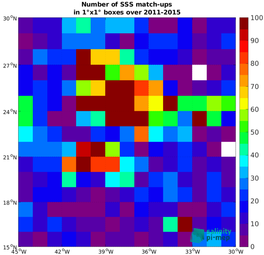
Figure 4: Number of SSS match-ups between Argo SSS and the Aquarius SSS L4 OI v5 - Weekly (IPRC) SSS product for the SPURS 1 Pi-MEP region over 1^\circ \times 1^\circ boxes and for the full satellite product period.
