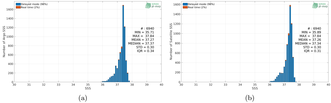
Figure 2: Histograms of SSS from Argo (a) and Aquarius SSS L4 OI v5 - Weekly (IPRC) (b) considering all match-up pairs per bins of 0.1 over the SPURS 1 Pi-MEP region and for the full satellite product period.
