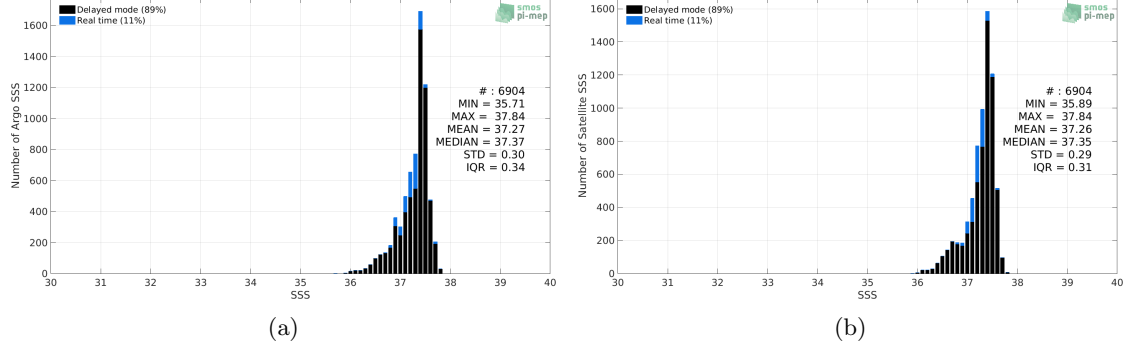
Figure 2: Histograms of SSS from Argo (a) and Aquarius SSS L4 OI v5 - Weekly (IPRC) (b) considering all match-up pairs per bins of 0.1 over the SPURS 1 Pi-MEP region and for the full satellite product period.
