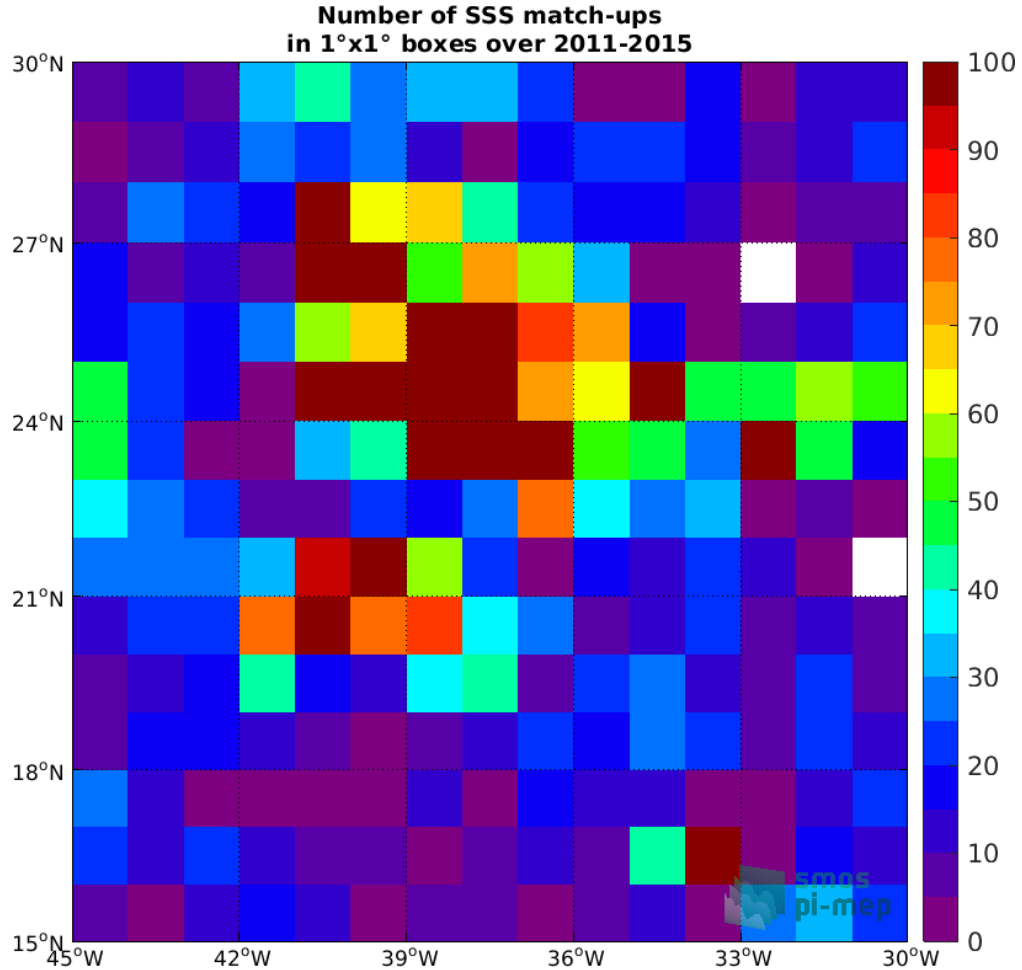
Figure 4: Number of SSS match-ups between Argo SSS and the Aquarius SSS L4 OI v5 - Weekly (IPRC) SSS product for the SPURS 1 Pi-MEP region over 1°x1° boxes and for the full satellite product period.
