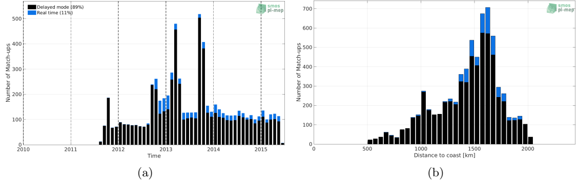
Figure 1: Number of match-ups between Argo and Aquarius SSS L4 OI v5 - Weekly (IPRC) SSS as a function of time (a) and as function of the distance to coast (b) over the SPURS 1 Pi-MEP region and for the full satellite product period.
