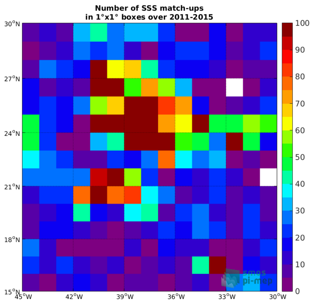
Figure 4: Number of SSS match-ups between Argo SSS and the Aquarius-L4-IPRC-V5-WEEKLY SSS product for the SPURS 1 Pi-MEP region over 1°x1° boxes and for the full satellite product period.
