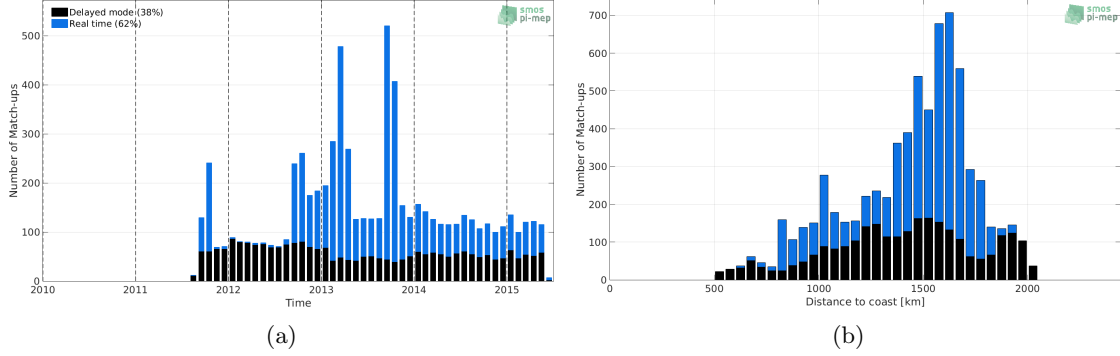
Figure 1: Number of match-ups between Argo and Aquarius-L4-IPRC-V5-WEEKLY SSS as a function of time (a) and as function of the distance to coast (b) over the SPURS 1 Pi-MEP region and for the full satellite product period.
