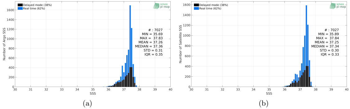
Figure 2: Histograms of SSS from Argo (a) and Aquarius-L4-IPRC-V5-WEEKLY (b) considering all match-up pairs per bins of 0.1 over the SPURS 1 Pi-MEP region and for the full satellite product period.
