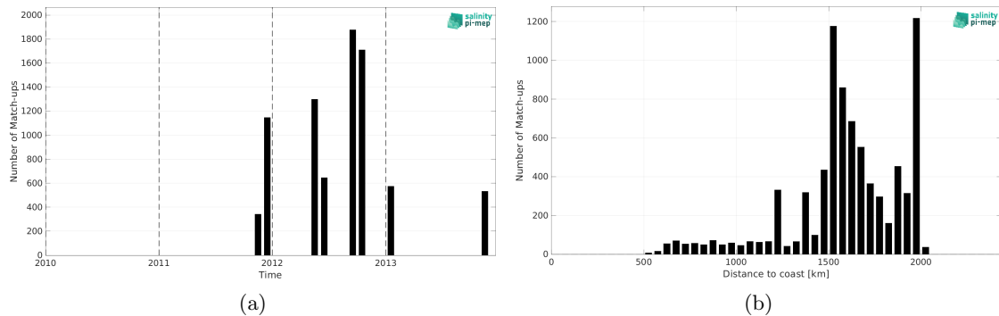
Figure 1: Number of match-ups between TSG (SAMOS) and Aquarius SSS L4 OI v5 - Monthly (IPRC) SSS as a function of time (a) and as function of the distance to coast (b) over the SPURS 1 Pi-MEP region and for the full satellite product period.
