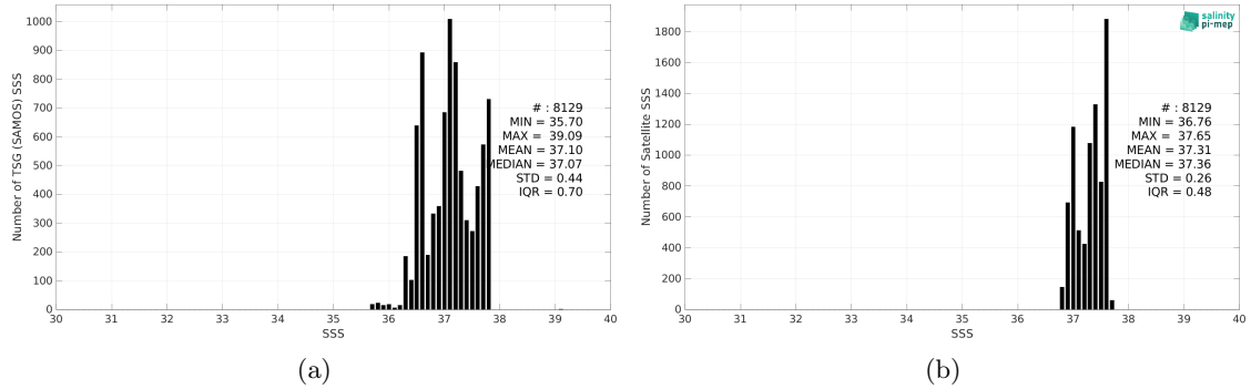
Figure 2: Histograms of SSS from TSG (SAMOS) (a) and Aquarius SSS L4 OI v5 - Monthly (IPRC) (b) considering all match-up pairs per bins of 0.1 over the SPURS 1 Pi-MEP region and for the full satellite product period.
