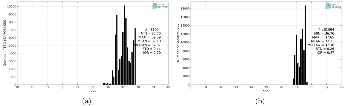
Figure 2: Histograms of SSS from TSG (SAMOS) (a) and Aquarius SSS L4 OI v5 - Monthly (IPRC) (b) considering all match-up pairs per bins of 0.1 over the SPURS 1 Pi-MEP region and for the full satellite product period.
