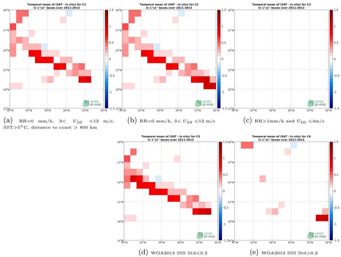
Figure 12: Temporal mean gridded over spatial boxes of size 1^\circ \times 1^\circ of \Delta\text{SSS} (Aquarius SSS L4 OI v5 - Monthly (IPRC) - TSG (SAMOS)) for 5 different subdatasets corresponding to:RR=0 mm/h, 3 < U_{10} < 12 m/s, SST >5^\circ\text{C} , distance to coast > 800 km (a), RR=0 mm/h, 3 < U_{10} < 12 m/s (b), RR >1 mm/h and U_{10} < 4 m/s (c), WOA2013 SSS Std <0.2 (d), WOA2013 SSS Std >0.2 (e).
