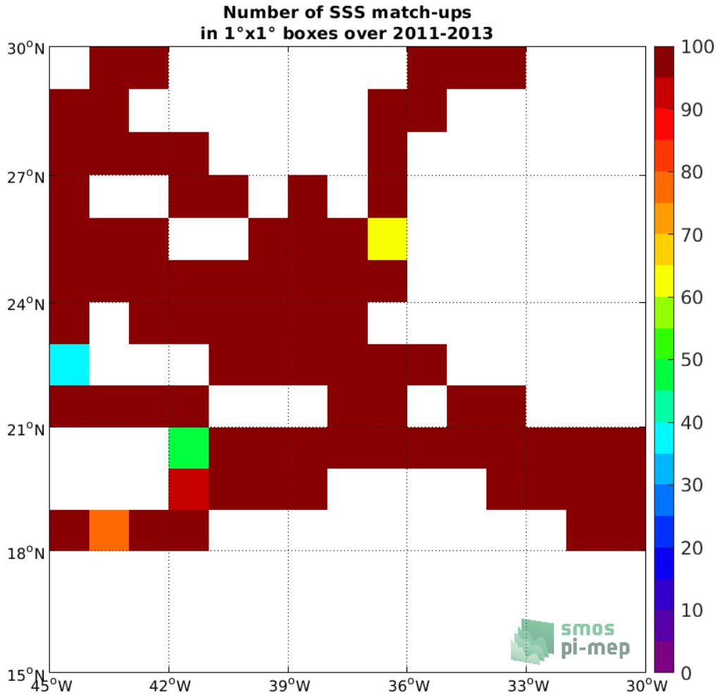
Figure 4: Number of SSS match-ups between TSG (SAMOS) SSS and the Aquarius SSS L4 OI v5 - Monthly (IPRC) SSS product for the SPURS 1 Pi-MEP region over 1^\circ \times 1^\circ boxes and for the full satellite product period.
