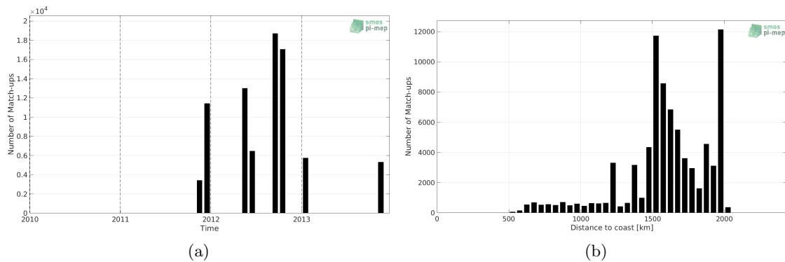
Figure 1: Number of match-ups between TSG (SAMOS) and Aquarius SSS L4 OI v5 - Monthly (IPRC) SSS as a function of time (a) and as function of the distance to coast (b) over the SPURS 1 Pi-MEP region and for the full satellite product period.
