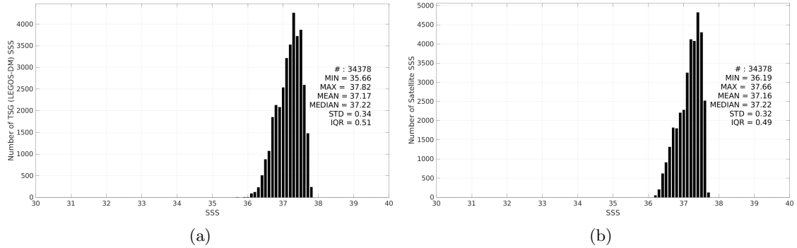
Figure 3: Histograms of SSS from TSG (LEGOS-DM) (a) and Aquarius SSS L4 OI v5 - Monthly (IPRC) (b) considering all match-up pairs per bins of 0.1 over the SPURS 1 Pi-MEP region and for the full satellite product period.
