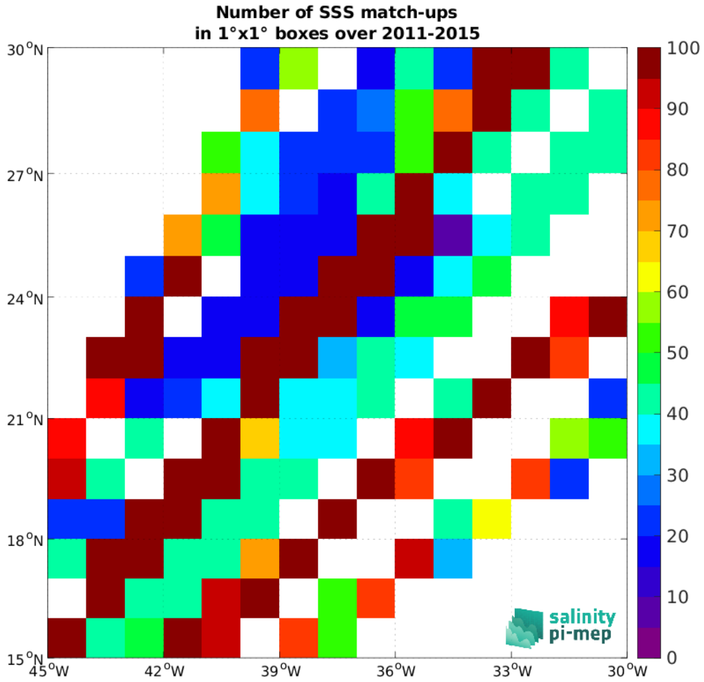
Figure 5: Number of SSS match-ups between TSG (LEGOS-DM) SSS and the Aquarius SSS L4 OI v5 - Monthly (IPRC) SSS product for the SPURS 1 Pi-MEP region over 1°x1° boxes and for the full satellite product period.
