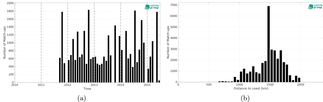
Figure 2: Number of match-ups between TSG (LEGOS-DM) and Aquarius SSS L4 OI v5 - Monthly (IPRC) SSS as a function of time (a) and as function of the distance to coast (b) over the SPURS 1 Pi-MEP region and for the full satellite product period.
