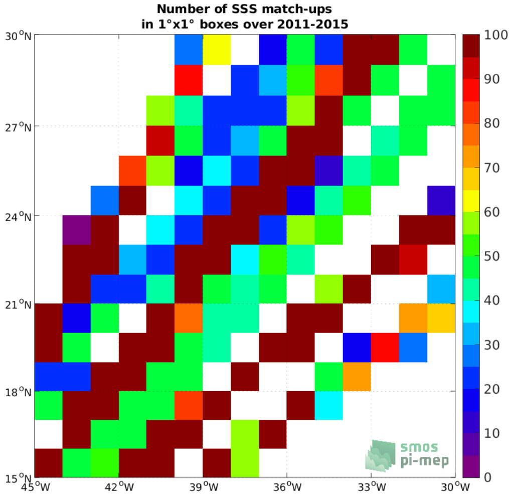
Figure 4: Number of SSS match-ups between TSG (LEGOS-DM) SSS and the Aquarius SSS L4 OI v5 - Monthly (IPRC) SSS product for the SPURS 1 Pi-MEP region over 1^\circ \times 1^\circ boxes and for the full satellite product period.
