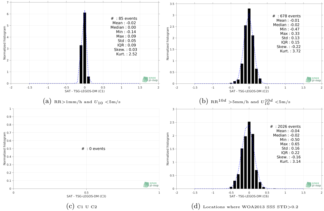
Figure 13: Normalized histogram of \Delta\text{SSS} (Aquarius-L4-IPRC-V5-MONTHLY - TSG-LEGOS-DM) for 6 different subdatasets corresponding to: RR > 1mm/h and U_{10} < 5\text{m/s} (a), RR^{10d} > 5\text{mm/h} and U_{10}^{10d} < 5\text{m/s} (b), C1 U C2 (c), Locations where WOA2013 SSS STD > 0.2 (d).
