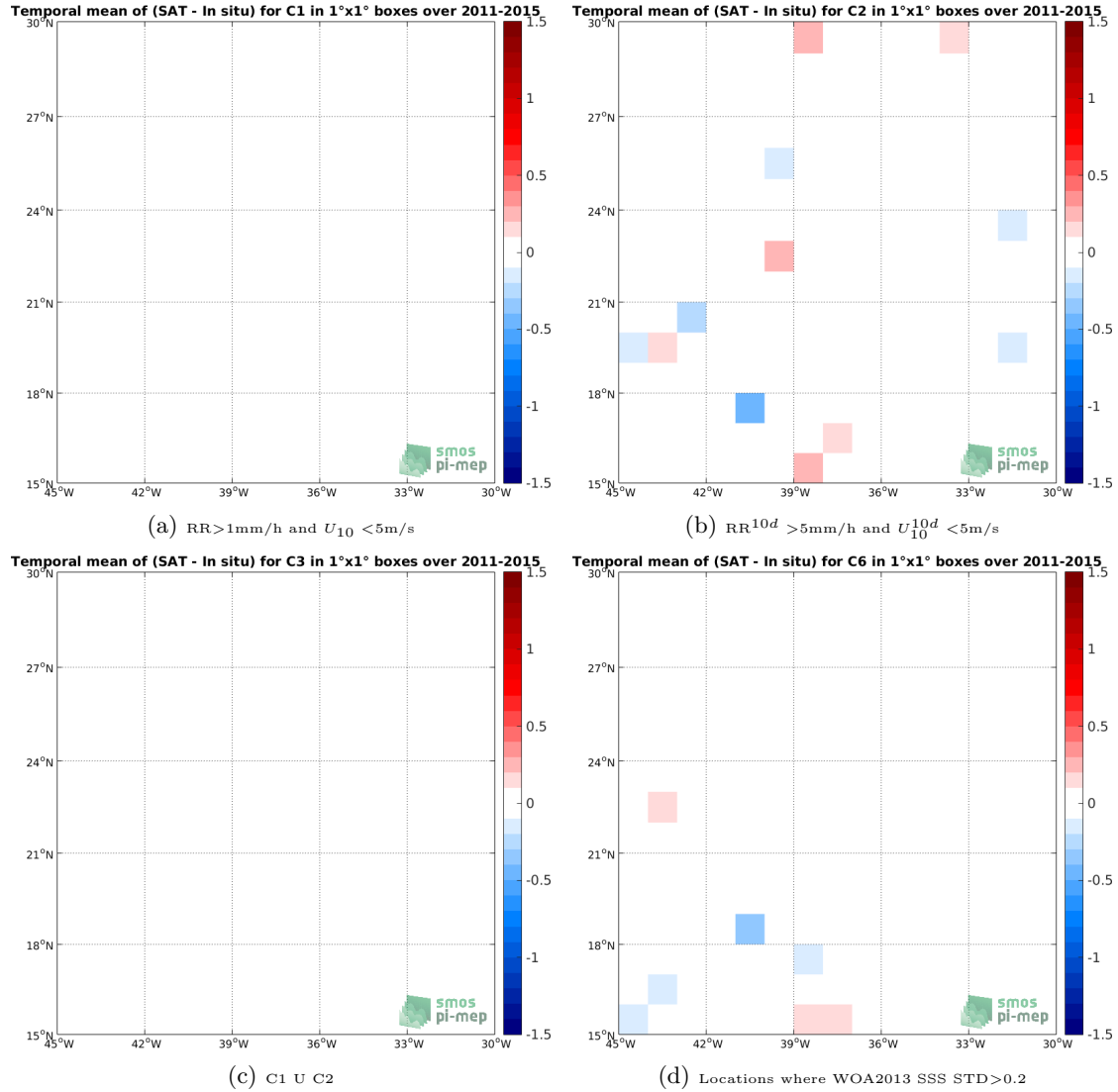
Figure 12: Temporal mean gridded over spatial boxes of size 1^\circ \times 1^\circ of \Delta SSS (Aquarius-L4-IPRC-V5-MONTHLY - TSG-LEGOS-DM) for 4 different subdatasets corresponding to: RR > 1\text{mm/h} and U_{10} < 5\text{m/s} (a), RR^{10d} > 5\text{mm/h} and U_{10}^{10d} < 5\text{m/s} (b), C1 U C2 (c), Locations where WOA2013 SSS STD > 0.2 (d).
