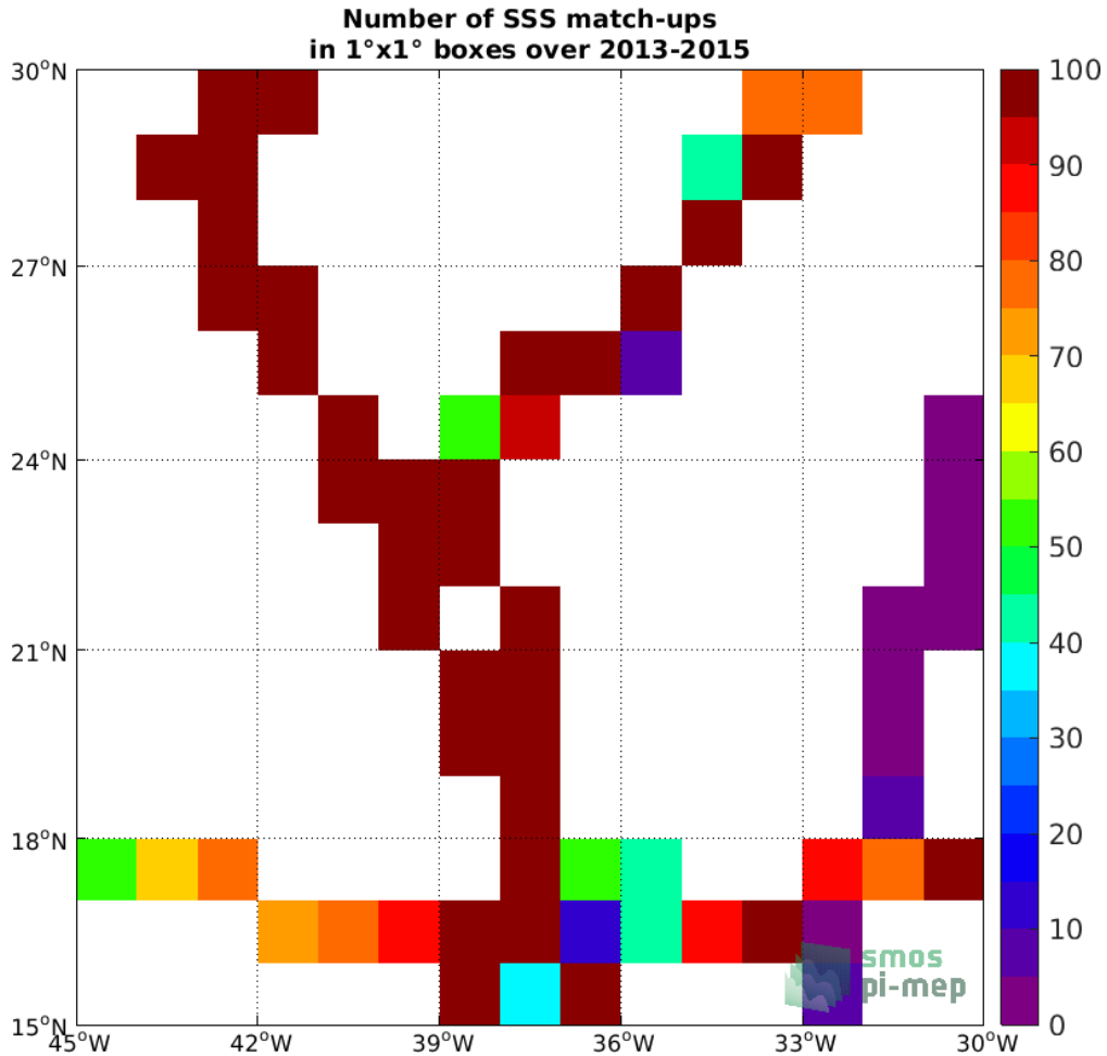
Figure 4: Number of SSS match-ups between TSG (GOSUD-Sailing-ship) SSS and the Aquarius SSS L4 OI v5 - Monthly (IPRC) SSS product for the SPURS 1 Pi-MEP region over 1°x1° boxes and for the full satellite product period.
