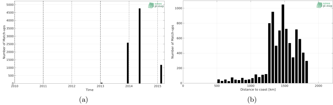
Figure 1: Number of match-ups between TSG (GOSUD-Sailing-ship) and Aquarius SSS L4 OI v5 - Monthly (IPRC) SSS as a function of time (a) and as function of the distance to coast (b) over the SPURS 1 Pi-MEP region and for the full satellite product period.
