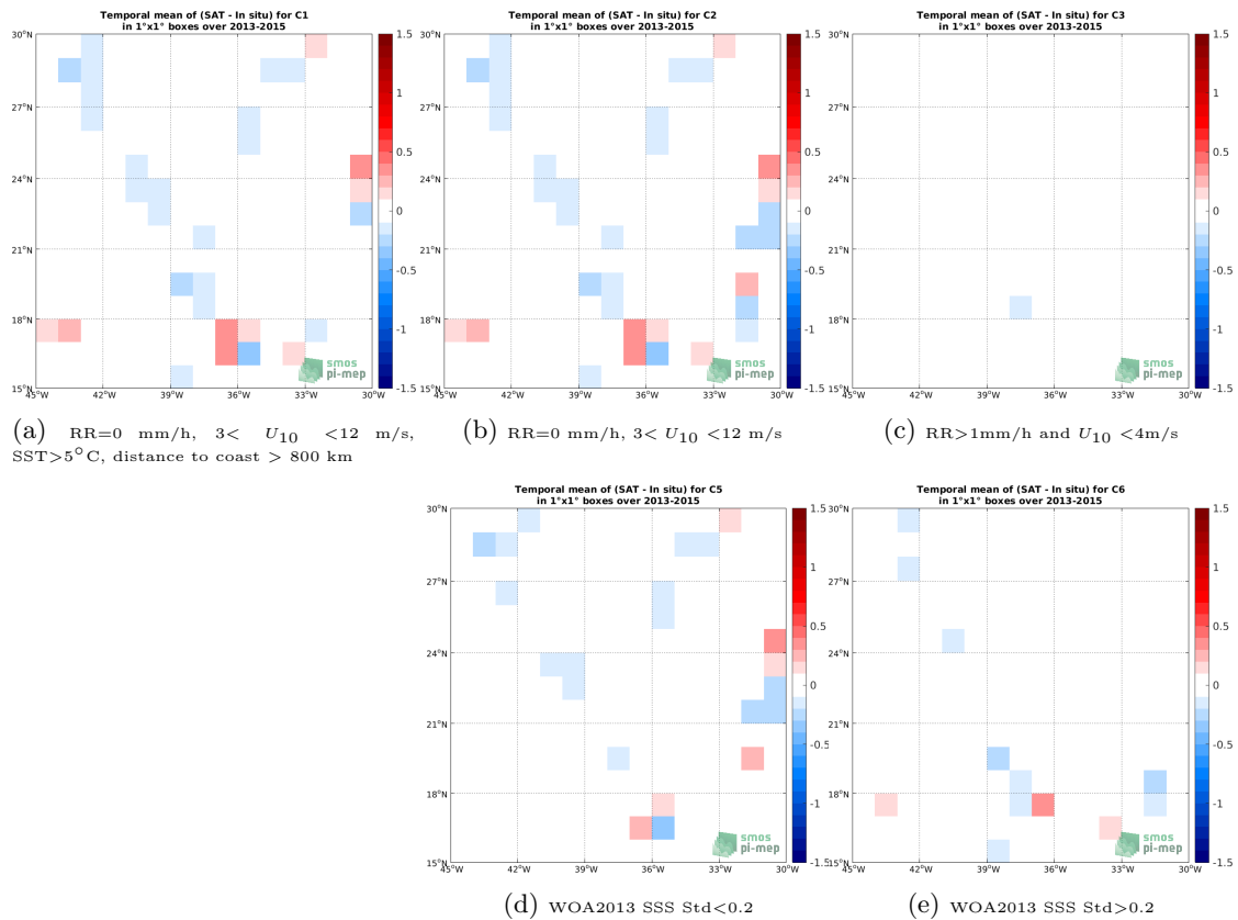
Figure 12: Temporal mean gridded over spatial boxes of size 1^\circ \times 1^\circ of \Delta\text{SSS} (Aquarius SSS L4 OI v5 - Monthly (IPRC) - TSG (GOSUD-Sailing-ship)) for 5 different subdatasets corresponding to:RR=0 mm/h, 3 < U_{10} < 12 m/s, SST>5°C, distance to coast > 800 km (a), RR=0 mm/h, 3 < U_{10} < 12 m/s (b), RR>1mm/h and U_{10} < 4 m/s (c), WOA2013 SSS Std<0.2 (d), WOA2013 SSS Std>0.2 (e).
