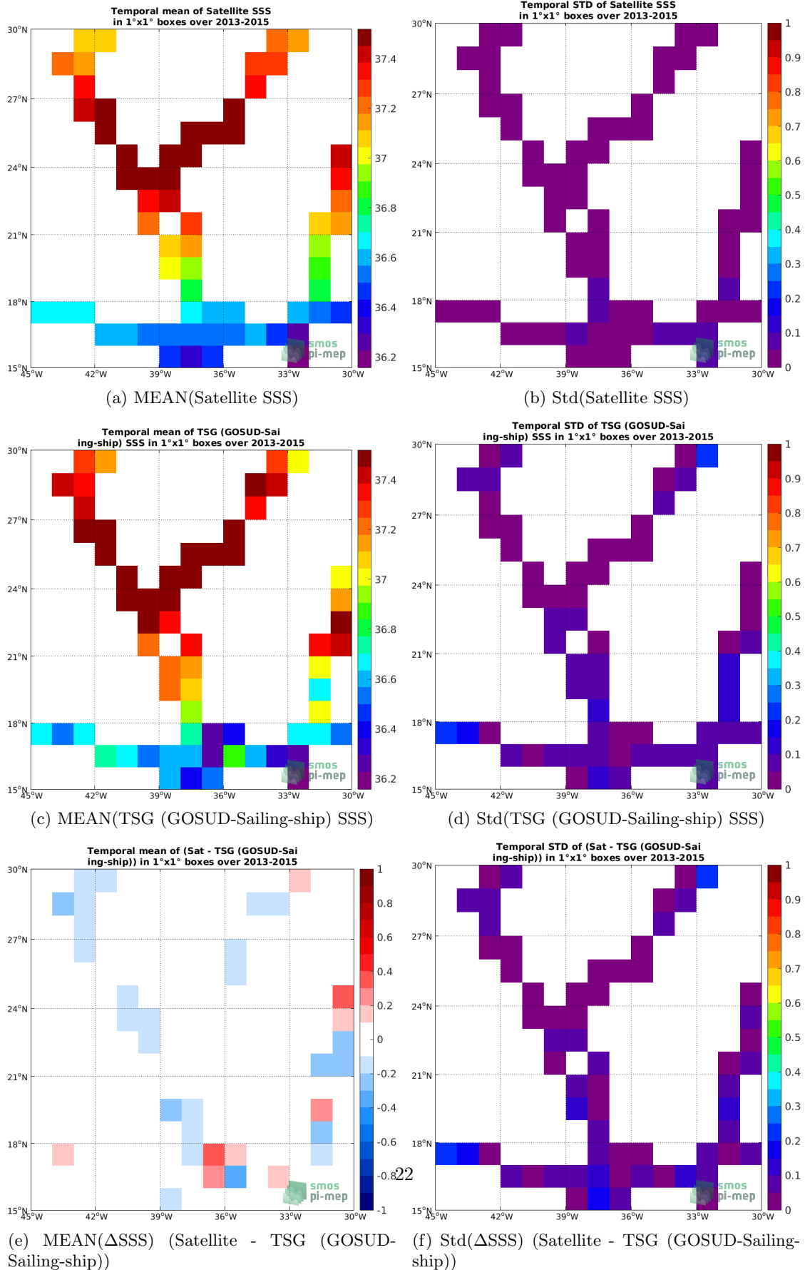
Figure 6: Temporal mean (left) and Std (right) of SSS from Aquarius SSS L4 OI v5 - Monthly (IPRC) (top), TSG (GOSUD-Sailing-ship) (middle), and of \Delta SSS (Satellite - TSG (GOSUD-Sailing-ship)). Only match-up pairs are used to generate these maps.
