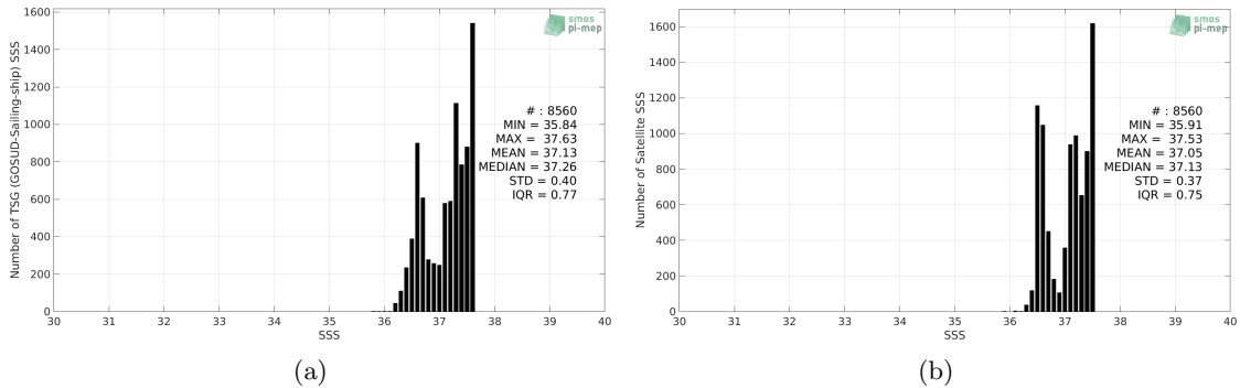
Figure 2: Histograms of SSS from TSG (GOSUD-Sailing-ship) (a) and Aquarius SSS L4 OI v5 - Monthly (IPRC) (b) considering all match-up pairs per bins of 0.1 over the SPURS 1 Pi-MEP region and for the full satellite product period.
