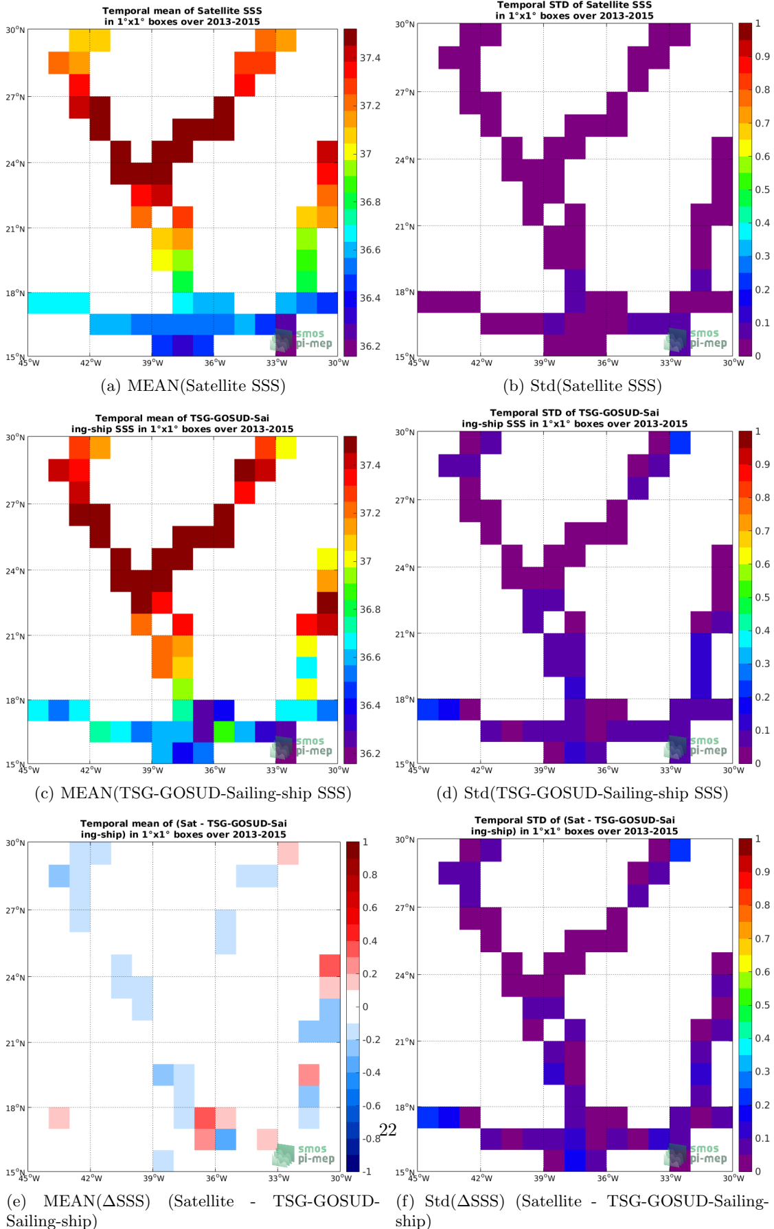
Figure 6: Temporal mean (left) and Std (right) of SSS from Aquarius-L4-IPRC-V5-MONTHLY (top), TSG-GOSUD-Sailing-ship (middle), and of \Delta SSS (Satellite - TSG-GOSUD-Sailing-ship). Only match-up pairs are used to generate these maps.
