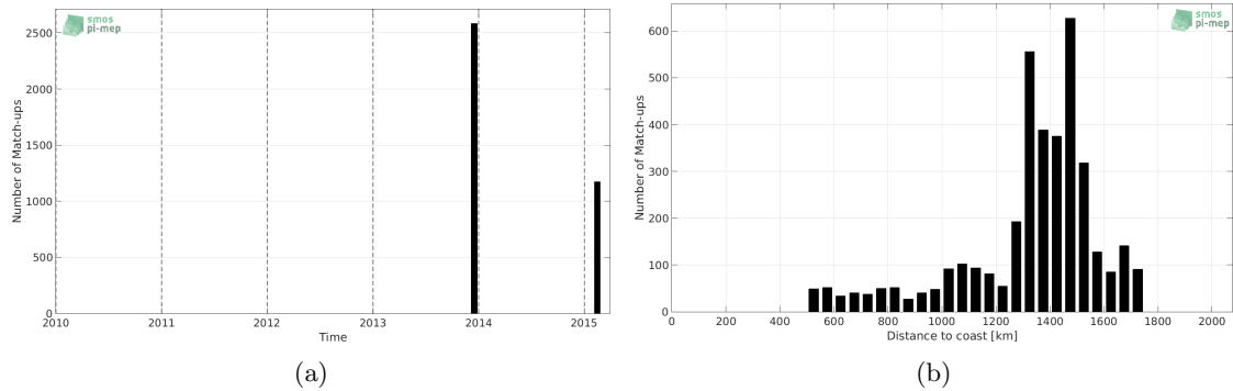
Figure 1: Number of match-ups between TSG-GOSUD-Sailing-ship and Aquarius-L4-IPRC-V5-MONTHLY SSS as a function of time (a) and as function of the distance to coast (b) over the SPURS 1 Pi-MEP region and for the full satellite product period.
