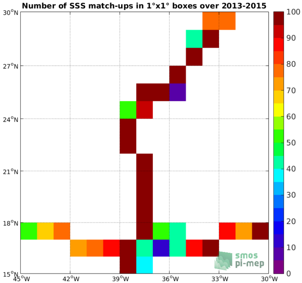
Figure 4: Number of SSS match-ups between TSG-GOSUD-Sailing-ship SSS and the Aquarius-L4-IPRC-V5-MONTHLY SSS product for the SPURS 1 Pi-MEP region over 1°x1° boxes and for the full satellite product period.
