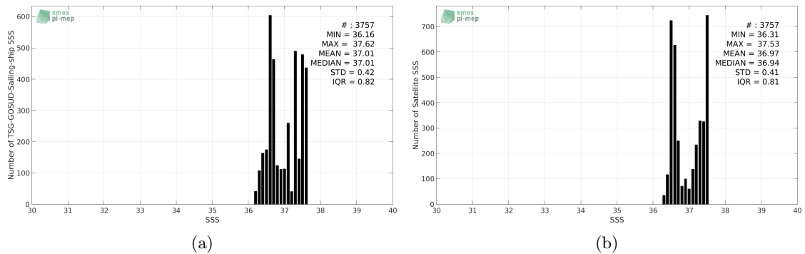
Figure 2: Histograms of SSS from TSG-GOSUD-Sailing-ship (a) and Aquarius-L4-IPRC-V5-MONTHLY (b) considering all match-up pairs per bins of 0.1 over the SPURS 1 Pi-MEP region and for the full satellite product period.
