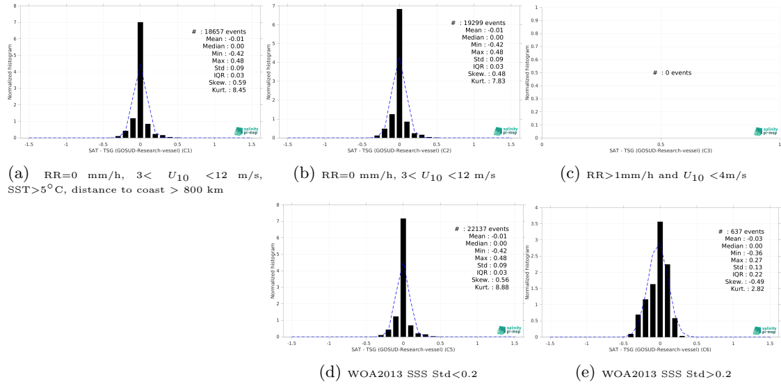
Figure 15: Normalized histogram of \Delta SSS (Aquarius SSS L4 OI v5 - Monthly (IPRC) - TSG (GOSUD-Research-vessel)) for 5 different subdatasets corresponding to: RR=0 mm/h, 3 < U_{10} < 12 m/s, SST > 5°C, distance to coast > 800 km (a), RR=0 mm/h, 3 < U_{10} < 12 m/s (b), RR > 1mm/h and U_{10} < 4 m/s (c), WOA2013 SSS Std < 0.2 (d), WOA2013 SSS Std > 0.2 (e).
