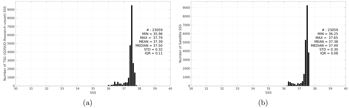
Figure 3: Histograms of SSS from TSG (GOSUD-Research-vessel) (a) and Aquarius SSS L4 OI v5 - Monthly (IPRC) (b) considering all match-up pairs per bins of 0.1 over the SPURS 1 Pi-MEP region and for the full satellite product period.
