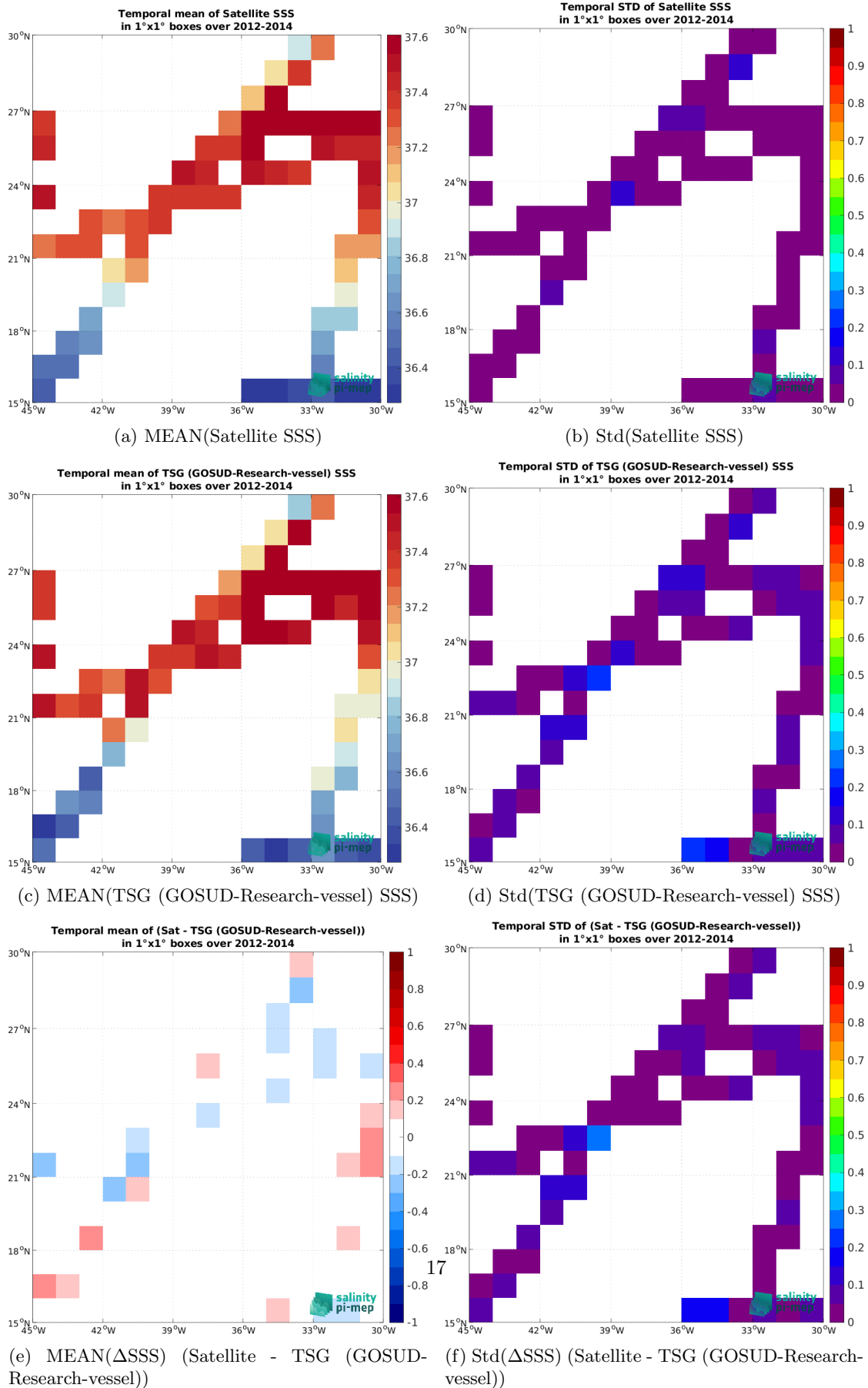
Figure 7: Temporal mean (left) and Std (right) of SSS from Aquarius SSS L4 OI v5 - Monthly (IPRC) (top), TSG (GOSUD-Research-vessel) (middle), and of \Delta SSS (Satellite - TSG (GOSUD-Research-vessel)). Only match-up pairs are used to generate these maps.
