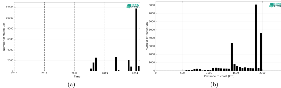
Figure 2: Number of match-ups between TSG (GOSUD-Research-vessel) and Aquarius SSS L4 OI v5 - Monthly (IPRC) SSS as a function of time (a) and as function of the distance to coast (b) over the SPURS 1 Pi-MEP region and for the full satellite product period.
