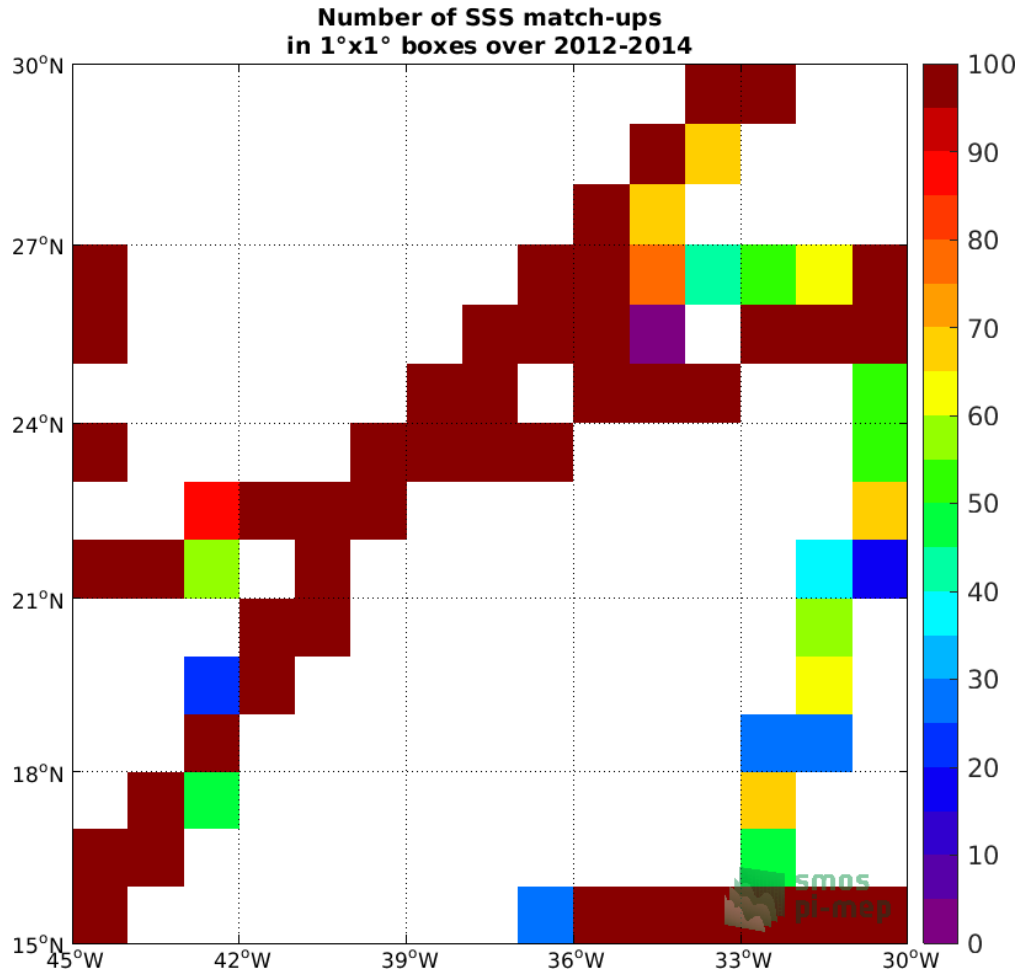
Figure 4: Number of SSS match-ups between TSG (GOSUD-Research-vessel) SSS and the Aquarius SSS L4 OI v5 - Monthly (IPRC) SSS product for the SPURS 1 Pi-MEP region over 1°x1° boxes and for the full satellite product period.
