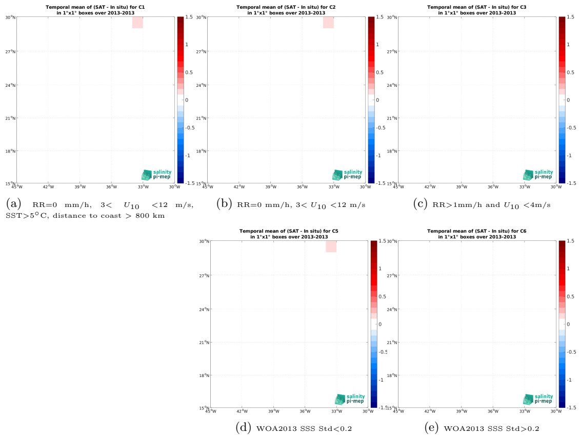
Figure 14: Temporal mean gridded over spatial boxes of size 1^\circ \times 1^\circ of \Delta SSS (Aquarius SSS L4 OI v5 - Monthly (IPRC) - TSG (CSIC-UTM)) for 5 different subdatasets corresponding to:RR=0 mm/h, 3 < U_{10} < 12 m/s, SST>5°C, distance to coast > 800 km (a), RR=0 mm/h, 3 < U_{10} < 12 m/s (b), RR>1mm/h and U_{10} < 4 m/s (c), WOA2013 SSS Std<0.2 (d), WOA2013 SSS Std>0.2 (e).
