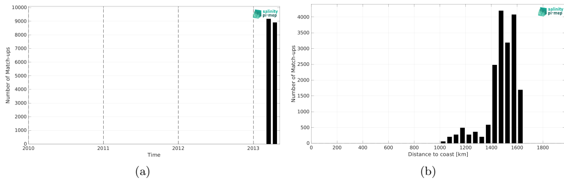
Figure 2: Number of match-ups between TSG (CSIC-UTM) and Aquarius SSS L4 OI v5 - Monthly (IPRC) SSS as a function of time (a) and as function of the distance to coast (b) over the SPURS 1 Pi-MEP region and for the full satellite product period.
