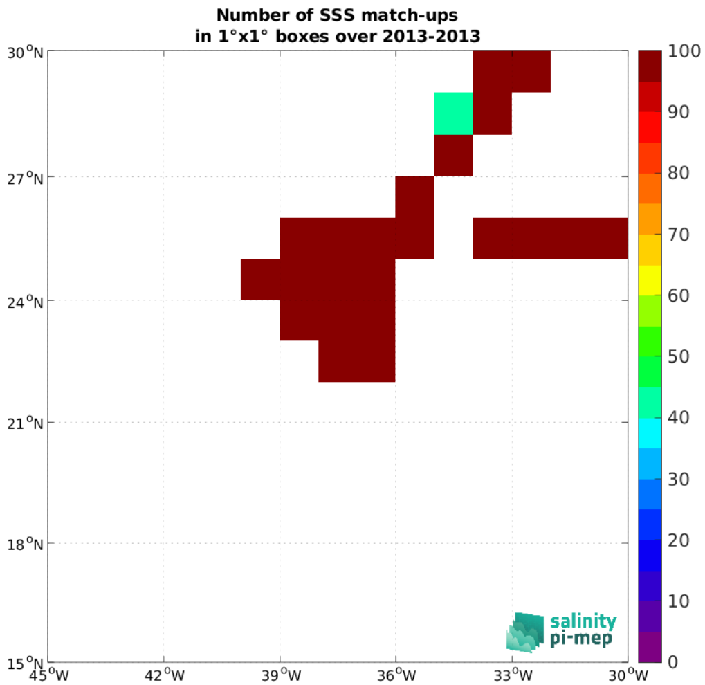
Figure 5: Number of SSS match-ups between TSG (CSIC-UTM) SSS and the Aquarius SSS L4 OI v5 - Monthly (IPRC) SSS product for the SPURS 1 Pi-MEP region over 1^\circ \times 1^\circ boxes and for the full satellite product period.
