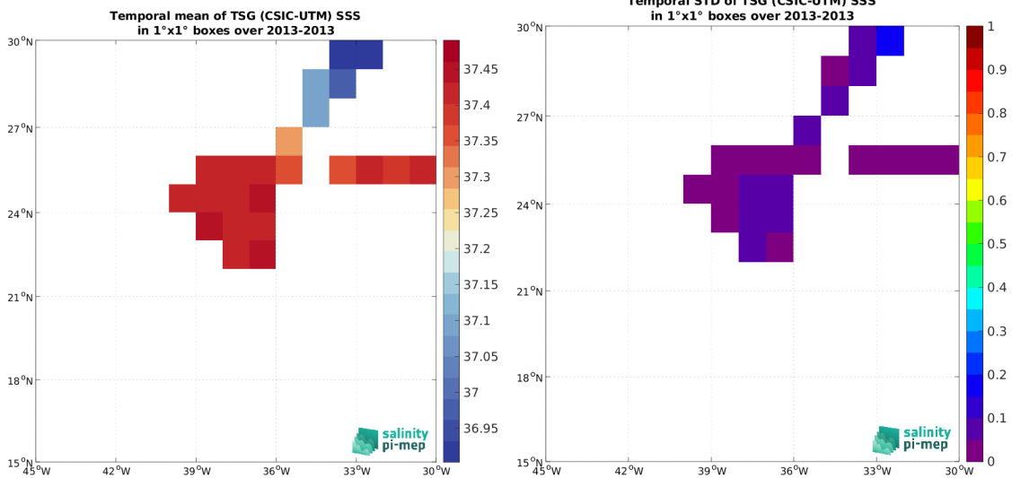
(c) MEAN(TSG (CSIC-UTM) SSS)
