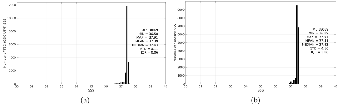
Figure 3: Histograms of SSS from TSG (CSIC-UTM) (a) and Aquarius SSS L4 OI v5 - Monthly (IPRC) (b) considering all match-up pairs per bins of 0.1 over the SPURS 1 Pi-MEP region and for the full satellite product period.
