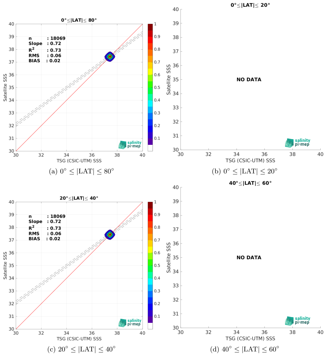
Figure 10: Contour maps of the concentration of Aquarius SSS L4 OI v5 - Monthly (IPRC) SSS (y-axis) versus TSG (CSIC-UTM) SSS (x-axis) at match-up pairs for different latitude bands. For each plot, the red line shows x=y . The black thin and dashed lines indicate a linear fit through the data cloud and the \pm 95\% confidence levels, respectively. The number match-up pairs n , the slope and R^2 coefficient of the linear fit, the root mean square (RMS) and the mean bias between satellite and in situ data are indicated for each latitude band in each plots.
