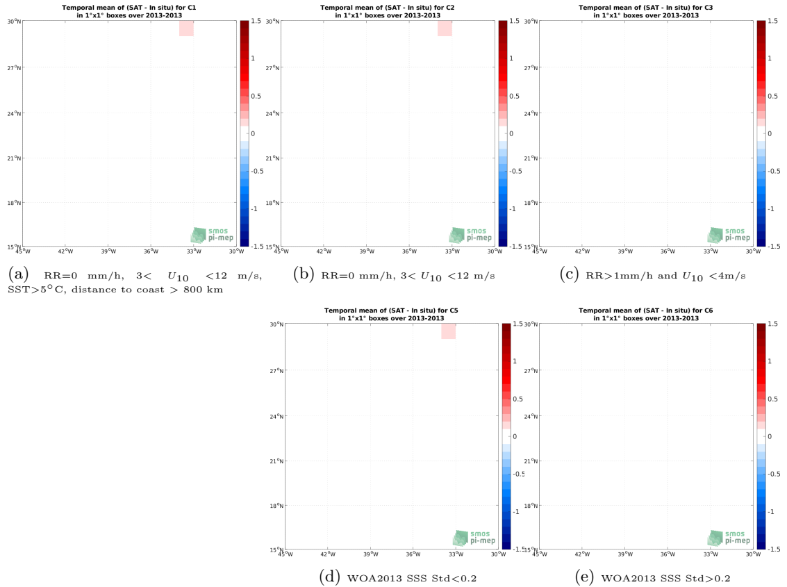
Figure 12: Temporal mean gridded over spatial boxes of size 1^{\circ}\times 1^{\circ} of \Delta\text{SSS} (Aquarius SSS L4 OI v5 - Monthly (IPRC) - TSG (CSIC-UTM)) for 5 different subdatasets corresponding to:RR=0 mm/h, 3 < U_{10} < 12 m/s, SST >5^{\circ}\text{C} , distance to coast > 800 km (a), RR=0 mm/h, 3 < U_{10} < 12 m/s (b), RR >1 mm/h and U_{10} < 4 m/s (c), WOA2013 SSS Std <0.2 (d), WOA2013 SSS Std >0.2 (e).
