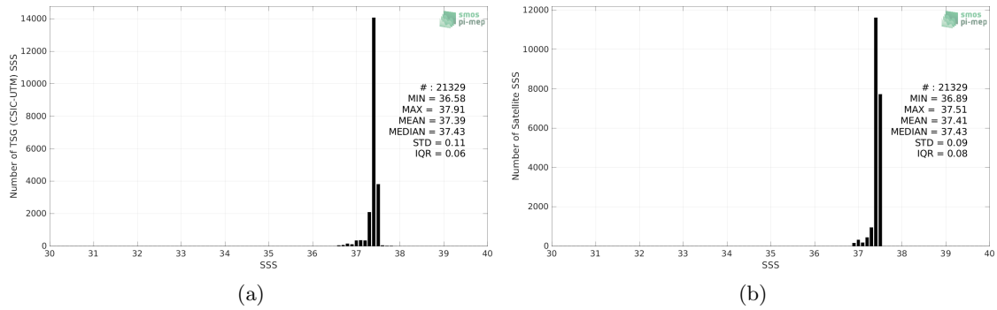
Figure 2: Histograms of SSS from TSG (CSIC-UTM) (a) and Aquarius SSS L4 OI v5 - Monthly (IPRC) (b) considering all match-up pairs per bins of 0.1 over the SPURS 1 Pi-MEP region and for the full satellite product period.
