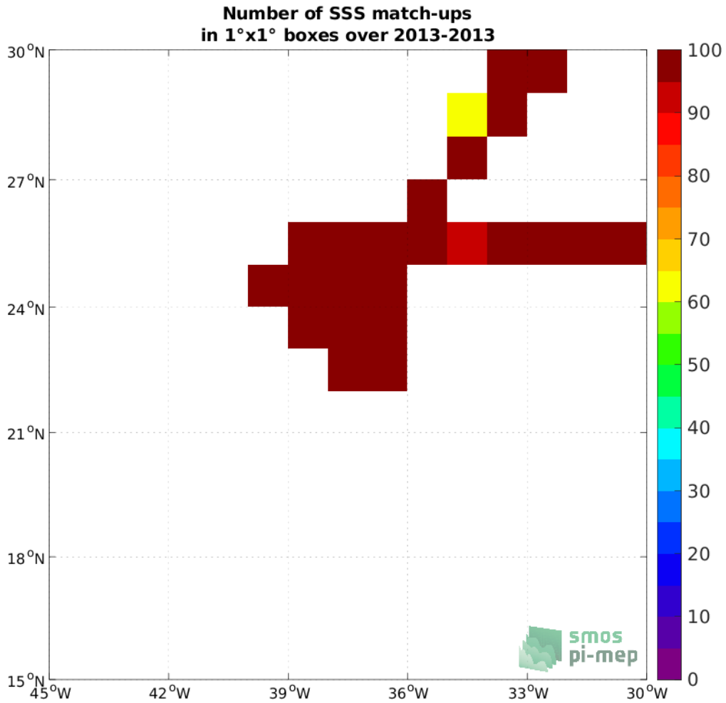
Figure 4: Number of SSS match-ups between TSG (CSIC-UTM) SSS and the Aquarius SSS L4 OI v5 - Monthly (IPRC) SSS product for the SPURS 1 Pi-MEP region over 1°x1° boxes and for the full satellite product period.
