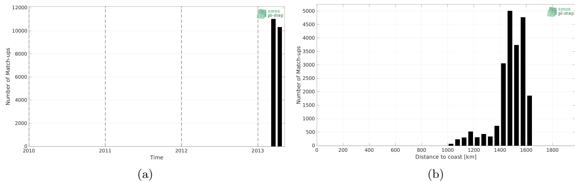
Figure 1: Number of match-ups between TSG (CSIC-UTM) and Aquarius SSS L4 OI v5 - Monthly (IPRC) SSS as a function of time (a) and as function of the distance to coast (b) over the SPURS 1 Pi-MEP region and for the full satellite product period.
