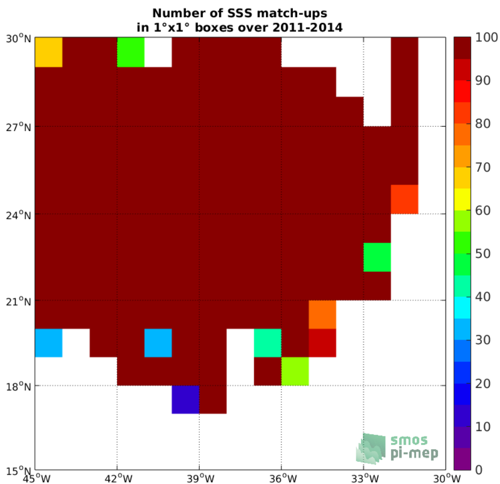
Figure 3: Number of SSS match-ups between Surface drifters SSS and the Aquarius-L4-IPRC-V5-MONTHLY SSS product for the SPURS 1 Pi-MEP region over 1°x1° boxes and for the full satellite product period.
