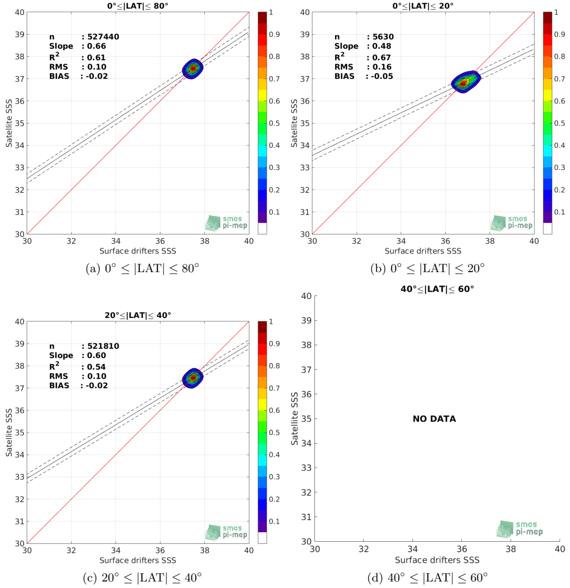
Figure 8: Contour maps of the concentration of Aquarius-L4-IPRC-V5-MONTHLY SSS (y-axis) versus Surface drifters SSS (x-axis) at match-up pairs for different latitude bands. For each plot, the red line shows x=y . The black thin and dashed lines indicate a linear fit through the data cloud and the \pm 95\% confidence levels, respectively. The number match-up pairs n , the slope and R^2 coefficient of the linear fit, the root mean square (RMS) and the mean bias between satellite and in situ data are indicated for each latitude band in each plots.
