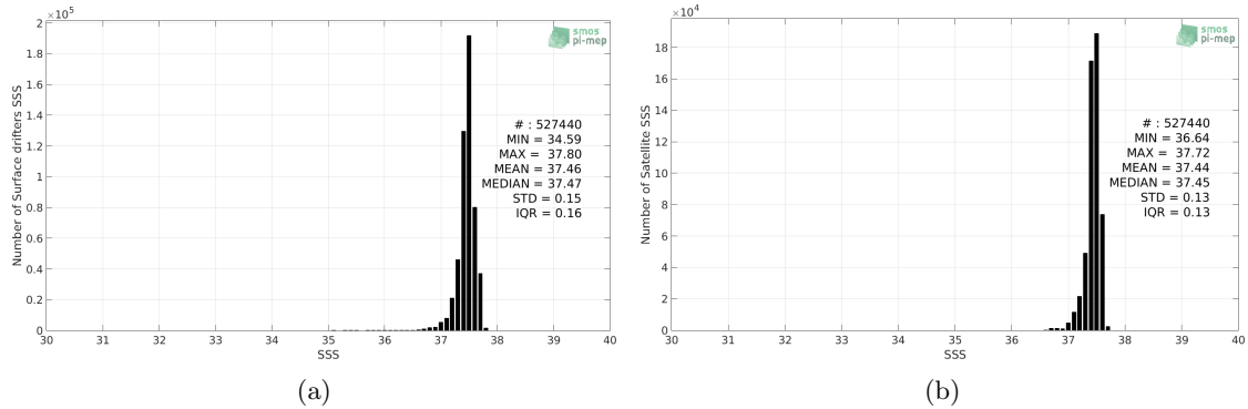
Figure 2: Histograms of SSS from Surface drifters (a) and Aquarius-L4-IPRC-V5-MONTHLY (b) considering all match-up pairs per bins of 0.1 over the SPURS 1 Pi-MEP region and for the full satellite product period.
