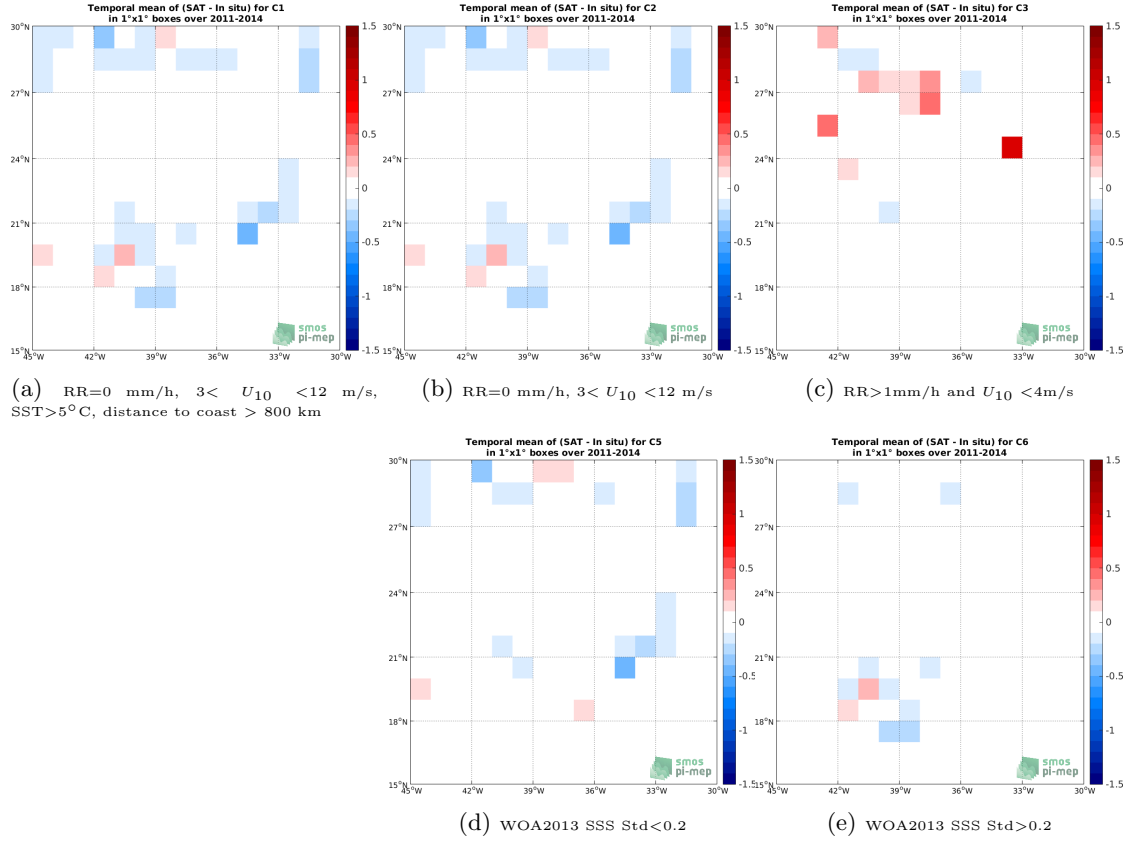
Figure 11: Temporal mean gridded over spatial boxes of size 1^\circ \times 1^\circ of \Delta SSS (Aquarius-L4-IPRC-V5-MONTHLY - Surface drifters) for 5 different subdatasets corresponding to: RR=0 mm/h, 3 < U_{10} < 12 m/s, SST >5^\circ C, distance to coast > 800 km (a), RR=0 mm/h, 3 < U_{10} < 12 m/s (b), RR >1 mm/h and U_{10} < 4 m/s (c), WOA2013 SSS Std <0.2 (d), WOA2013 SSS Std >0.2 (e).
