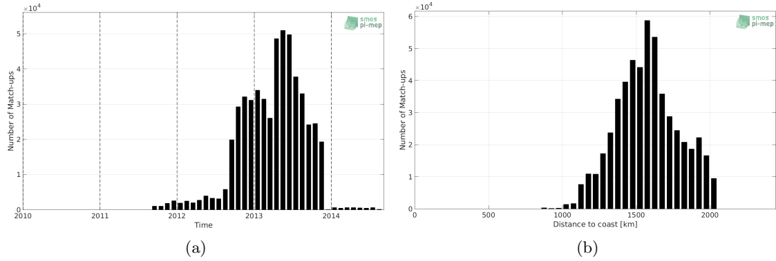
Figure 1: Number of match-ups between Surface drifters and Aquarius-L4-IPRC-V5-MONTHLY SSS as a function of time (a) and as function of the distance to coast (b) over the SPURS 1 Pi-MEP region and for the full satellite product period.
