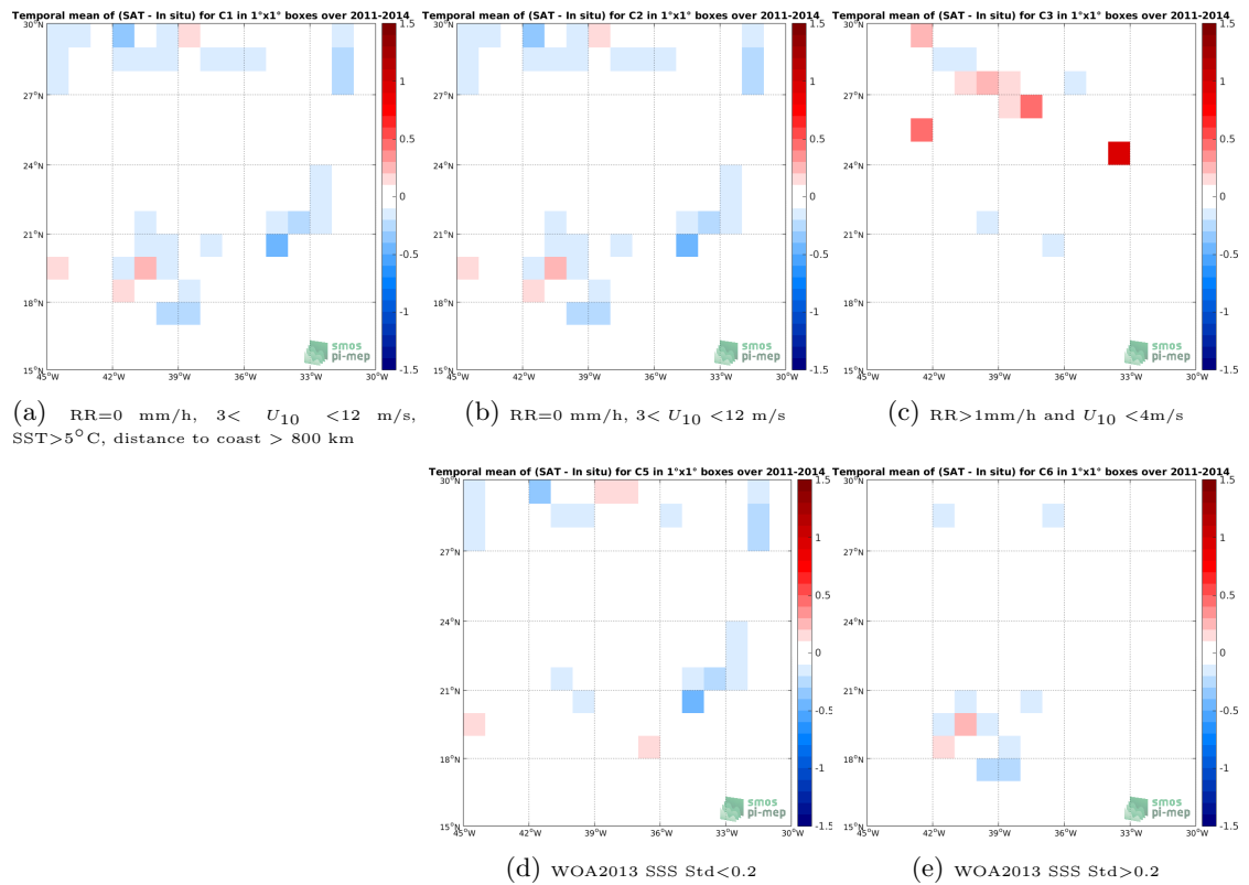
Figure 11: Temporal mean gridded over spatial boxes of size 1^\circ \times 1^\circ of \Delta SSS (Aquarius-L4-IPRC-V5-MONTHLY - Surface drifters) for 5 different subdatasets corresponding to: RR=0 mm/h, 3 < U_{10} < 12 m/s, SST > 5^\circ C , distance to coast > 800 km (a), RR=0 mm/h, 3 < U_{10} < 12 m/s (b), RR > 1 mm/h and U_{10} < 4 m/s (c), WOA2013 SSS Std < 0.2 (d), WOA2013 SSS Std > 0.2 (e).
