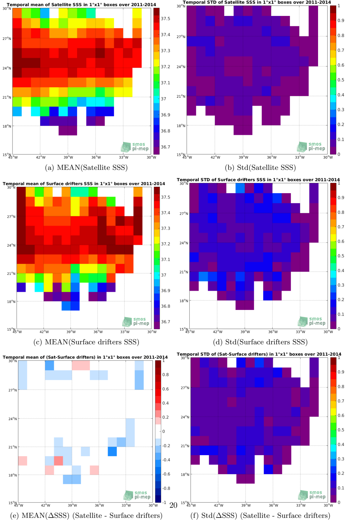
Figure 5: Temporal mean (left) and Std (right) of SSS from Aquarius-L4-IPRC-V5-MONTHLY (top), Surface drifters (middle), and of \Delta SSS (Satellite - Surface drifters). Only match-up pairs are used to generate these maps.
