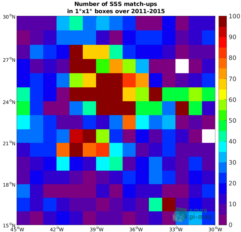
Figure 4: Number of SSS match-ups between Argo SSS and the Aquarius SSS L4 OI v5 - Monthly (IPRC) SSS product for the SPURS 1 Pi-MEP region over 1^\circ \times 1^\circ boxes and for the full satellite product period.
