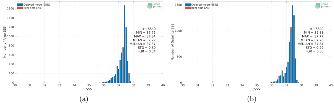
Figure 2: Histograms of SSS from Argo (a) and Aquarius SSS L4 OI v5 - Monthly (IPRC) (b) considering all match-up pairs per bins of 0.1 over the SPURS 1 Pi-MEP region and for the full satellite product period.
