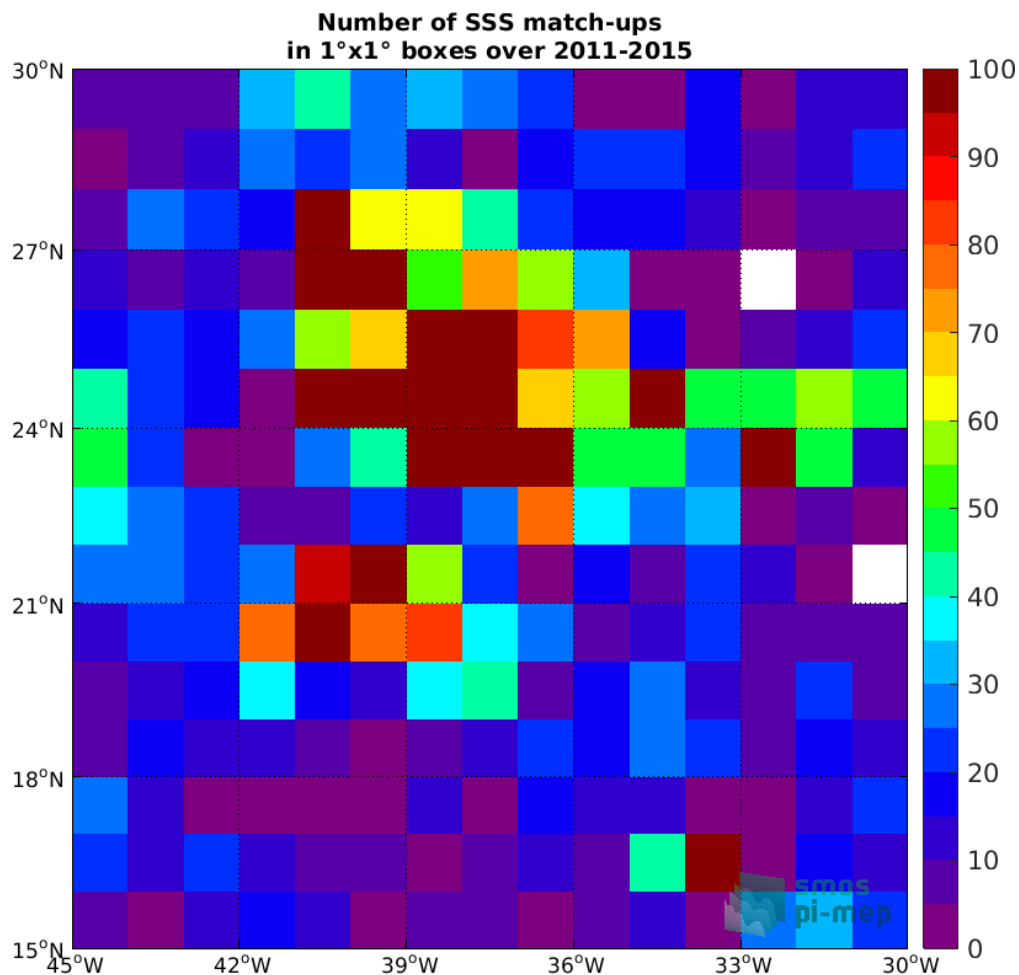
Figure 4: Number of SSS match-ups between Argo SSS and the Aquarius SSS L4 OI v5 - Monthly (IPRC) SSS product for the SPURS 1 Pi-MEP region over 1°x1° boxes and for the full satellite product period.
