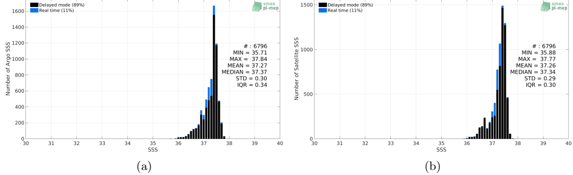
Figure 2: Histograms of SSS from Argo (a) and Aquarius SSS L4 OI v5 - Monthly (IPRC) (b) considering all match-up pairs per bins of 0.1 over the SPURS 1 Pi-MEP region and for the full satellite product period.
