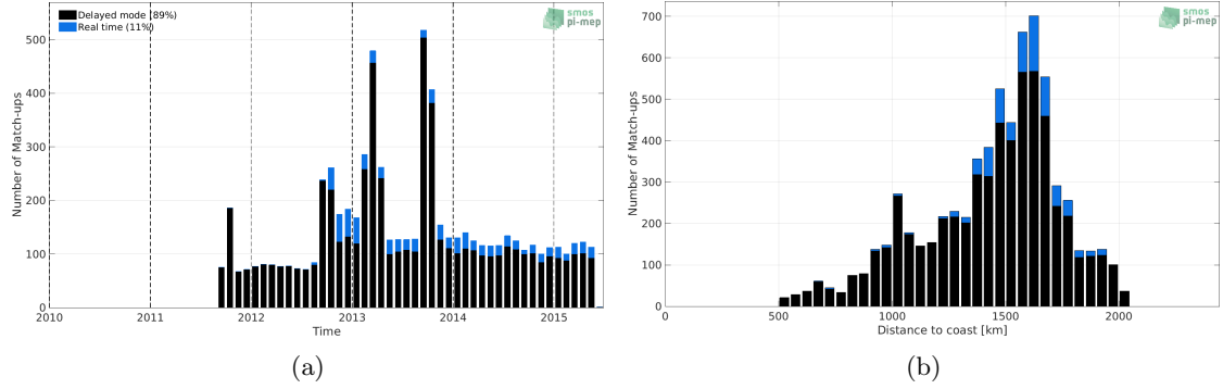
Figure 1: Number of match-ups between Argo and Aquarius SSS L4 OI v5 - Monthly (IPRC) SSS as a function of time (a) and as function of the distance to coast (b) over the SPURS 1 Pi-MEP region and for the full satellite product period.
