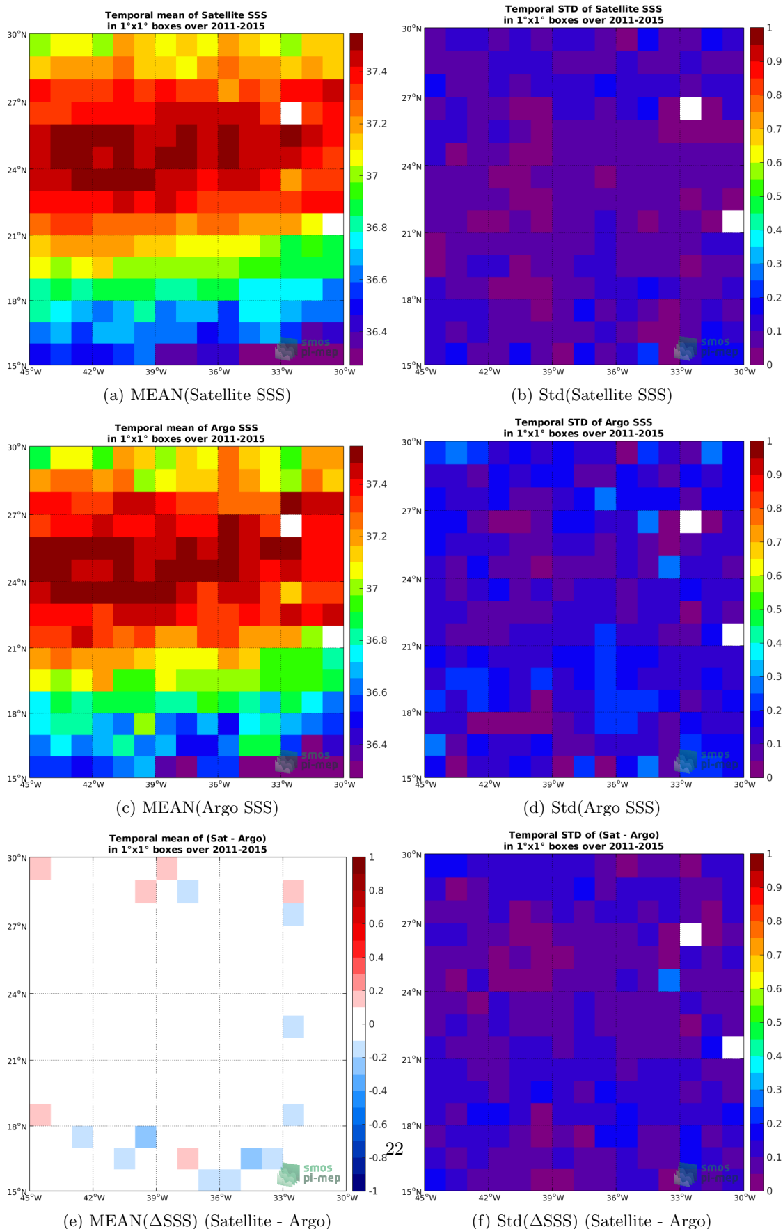
Figure 6: Temporal mean (left) and Std (right) of SSS from Aquarius-L4-IPRC-V5-MONTHLY (top), Argo (middle), and of ΔSSS (Satellite - Argo). Only match-up pairs are used to generate these maps.
