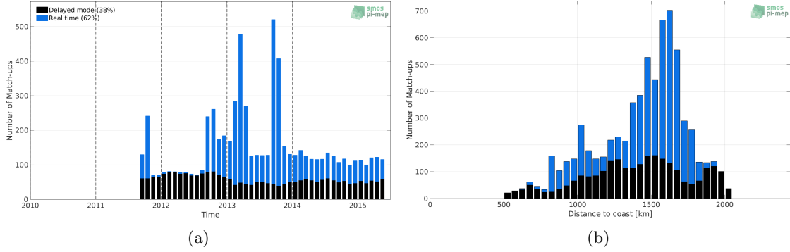
Figure 1: Number of match-ups between Argo and Aquarius-L4-IPRC-V5-MONTHLY SSS as a function of time (a) and as function of the distance to coast (b) over the SPURS 1 Pi-MEP region and for the full satellite product period.
