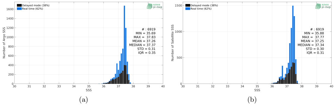
Figure 2: Histograms of SSS from Argo (a) and Aquarius-L4-IPRC-V5-MONTHLY (b) considering all match-up pairs per bins of 0.1 over the SPURS 1 Pi-MEP region and for the full satellite product period.
