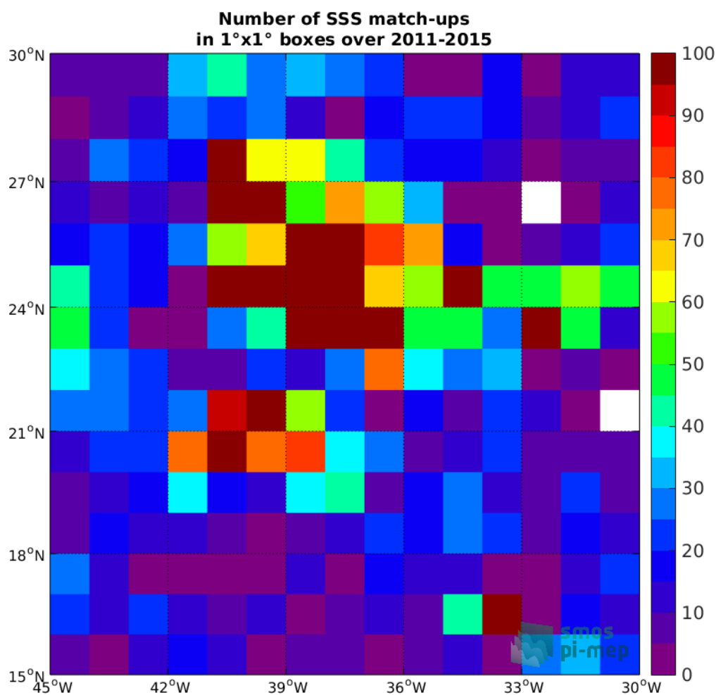
Figure 4: Number of SSS match-ups between Argo SSS and the Aquarius-L4-IPRC-V5-MONTHLY SSS product for the SPURS 1 Pi-MEP region over 1°x1° boxes and for the full satellite product period.
