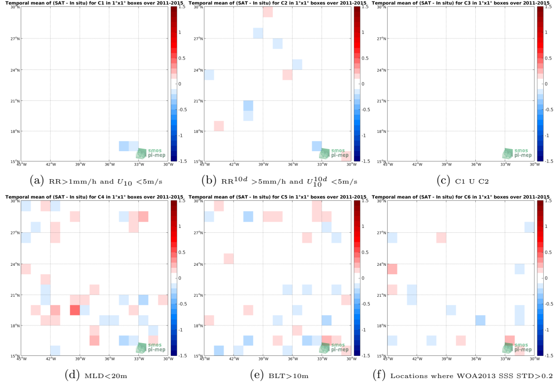
Figure 12: Temporal mean gridded over spatial boxes of size 1^\circ \times 1^\circ of \Delta\text{SSS} (Aquarius-L4-IPRC-V5-MONTHLY - Argo) for 6 different subdatasets corresponding to: \text{RR} > 1\text{mm/h} and U_{10} < 5\text{m/s} (a), \text{RR}^{10d} > 5\text{mm/h} and U_{10}^{10d} < 5\text{m/s} (b), C1 U C2 (c), \text{MLD} < 20\text{m} (d), \text{BLT} > 10\text{m} (e), Locations where WOA2013 SSS STD > 0.2 (f).
