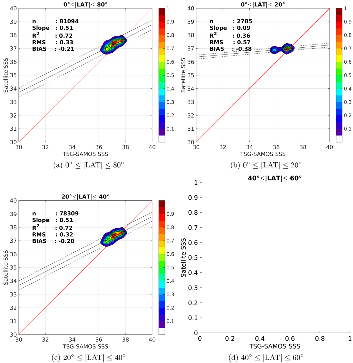
Figure 9: Contour maps of the concentration of Aquarius-L4-IPRC-V4-WEEKLY SSS (y-axis) versus TSG-SAMOS SSS (x-axis) at match-up pairs for different latitude bands. For each plot, the red line shows x=y . The black thin and dashed lines indicate a linear fit through the data cloud and the \pm 95\% confidence levels, respectively. The number match-up pairs n , the slope and R^2 coefficient of the linear fit, the root mean square (RMS) and the mean bias between satellite and in situ data are indicated for each latitude band in each plots.
