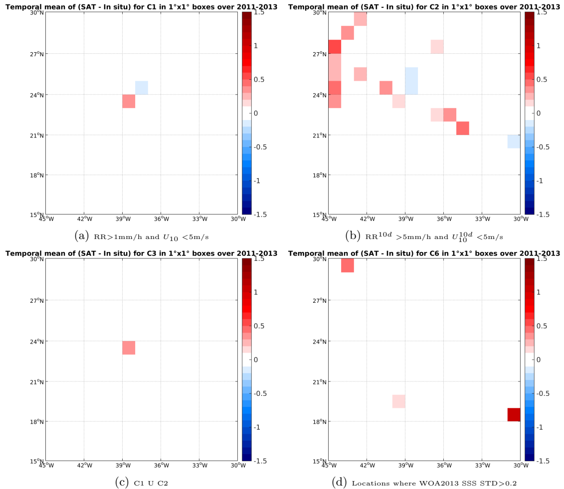
Figure 12: Temporal mean gridded over spatial boxes of size 1^\circ \times 1^\circ of \Delta SSS (Aquarius-L4-IPRC-V4-WEEKLY - TSG-SAMOS) for 4 different subdatasets corresponding to: RR > 1\text{mm/h} and U_{10} < 5\text{m/s} (a), RR^{10d} > 5\text{mm/h} and U_{10}^{10d} < 5\text{m/s} (b), C1 U C2 (c), Locations where WOA2013 SSS STD > 0.2 (d).
