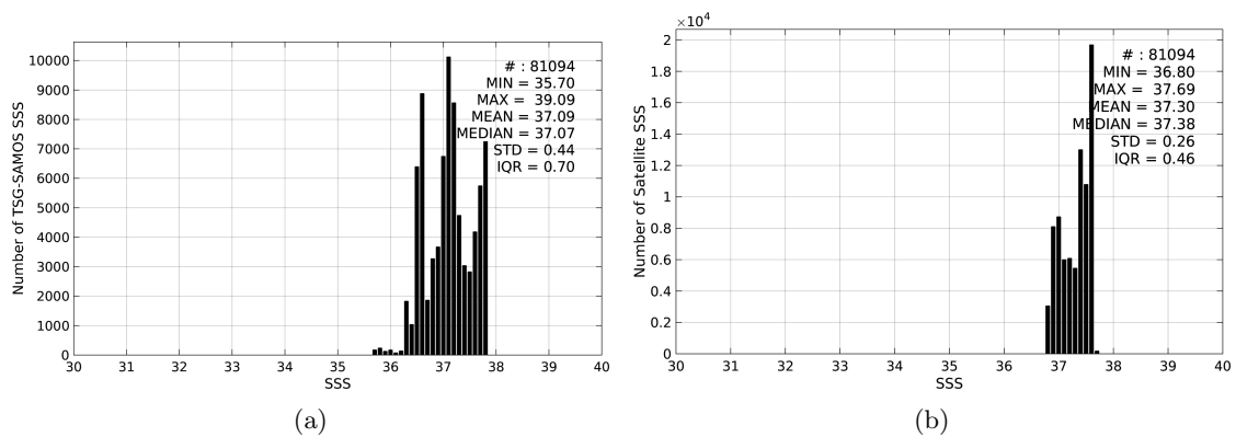
Figure 2: Histograms of SSS from TSG-SAMOS (a) and Aquarius-L4-IPRC-V4-WEEKLY (b) considering all match-up pairs per bins of 0.1 over the SPURS 1 Pi-MEP region and for the full satellite product period.
