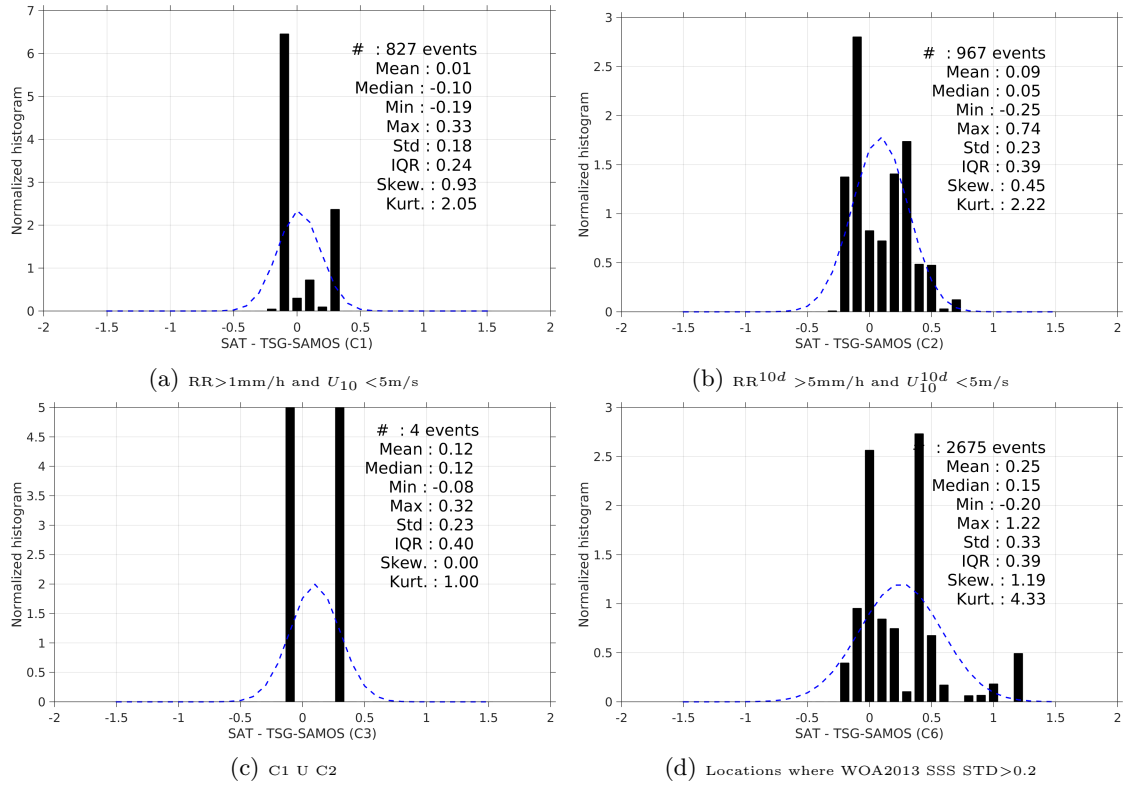
Figure 13: Normalized histogram of \Delta SSS (Aquarius-L4-IPRC-V4-WEEKLY - TSG-SAMOS) for 6 different subdatasets corresponding to: RR > 1mm/h and U_{10} < 5 m/s (a), RR^{10d} > 5 mm/h and U_{10}^{10d} < 5 m/s (b), C1 U C2 (c), Locations where WOA2013 SSS STD > 0.2 (d).
