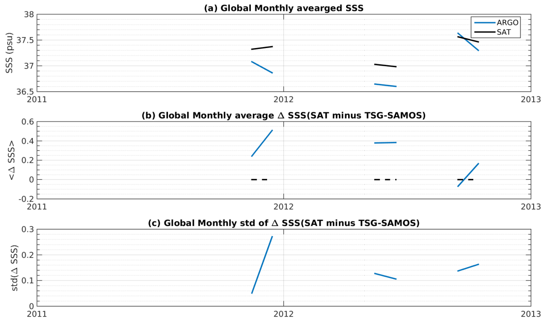
Figure 7: Time series of the monthly averaged mean SSS (top), mean \Delta SSS (Satellite - TSG-SAMOS) and STD of \Delta SSS (Satellite - TSG-SAMOS) over the SPURS 1 Pi-MEP region considering all match-ups collected by the Pi-MEP platform.
