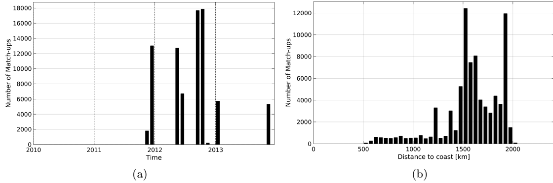
Figure 1: Number of match-ups between TSG-SAMOS and Aquarius-L4-IPRC-V4-WEEKLY SSS as a function of time (a) and as function of the distance to coast (b) over the SPURS 1 Pi-MEP region and for the full satellite product period.
