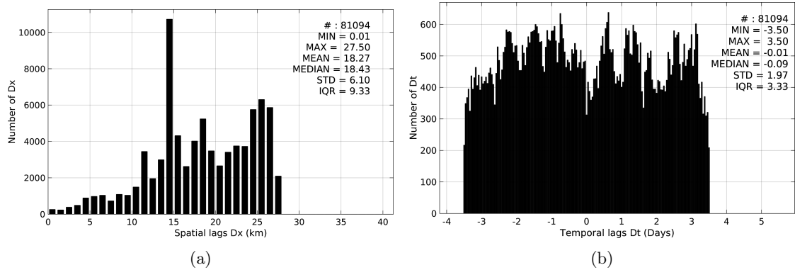
Figure 5: Histograms of the spatial (a) and temporal (b) lags between the time of the TSG-SAMOS measurements and the date of the corresponding Aquarius-L4-IPRC-V4-WEEKLY SSS product.
