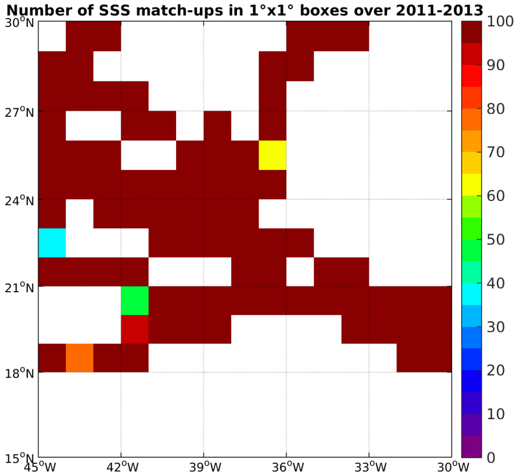
Figure 4: Number of SSS match-ups between TSG-SAMOS SSS and the Aquarius-L4-IPRC-V4-WEEKLY SSS product for the SPURS 1 Pi-MEP region over 1°x1° boxes and for the full satellite product period.
