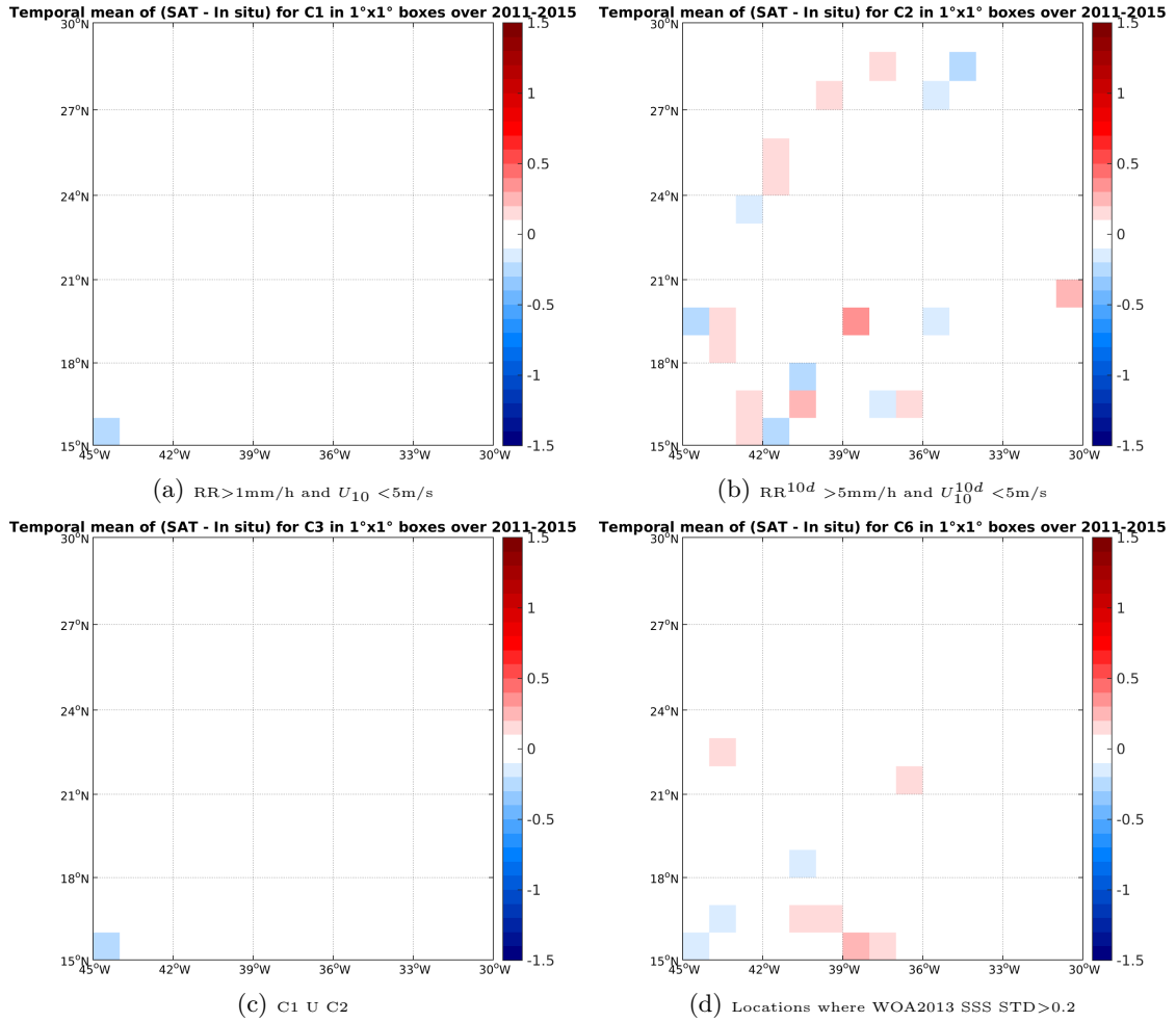
Figure 12: Temporal mean gridded over spatial boxes of size 1°x1° of \Delta SSS (Aquarius-L4-IPRC-V4-WEEKLY - TSG-LEGOS-DM) for 4 different subdatasets corresponding to: RR > 1\text{mm/h} and U_{10} < 5\text{m/s} (a), RR^{10d} > 5\text{mm/h} and U_{10}^{10d} < 5\text{m/s} (b), C1 U C2 (c), Locations where WOA2013 SSS STD > 0.2 (d).
