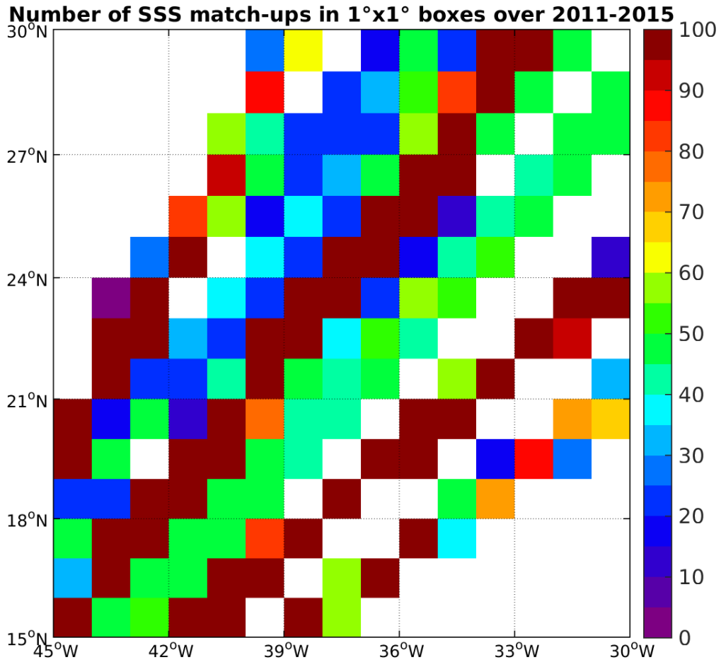
Figure 4: Number of SSS match-ups between TSG-LEGOS-DM SSS and the Aquarius-L4-IPRC-V4-WEEKLY SSS product for the SPURS 1 Pi-MEP region over 1°x1° boxes and for the full satellite product period.
