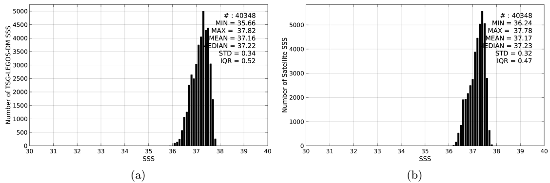
Figure 2: Histograms of SSS from TSG-LEGOS-DM (a) and Aquarius-L4-IPRC-V4-WEEKLY (b) considering all match-up pairs per bins of 0.1 over the SPURS 1 Pi-MEP region and for the full satellite product period.
