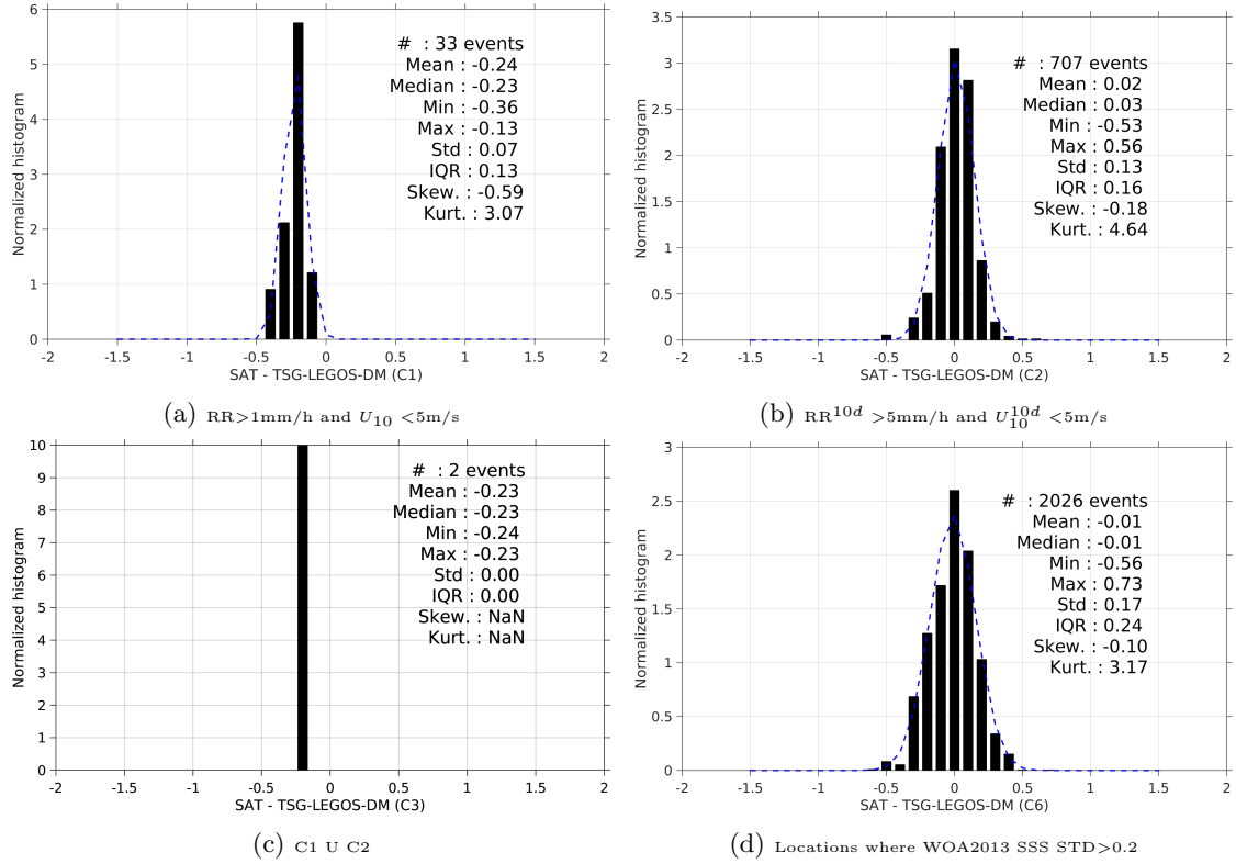
Figure 13: Normalized histogram of \Delta SSS (Aquarius-L4-IPRC-V4-WEEKLY - TSG-LEGOS-DM) for 6 different subdatasets corresponding to: RR > 1mm/h and U_{10} < 5 m/s (a), RR^{10d} > 5 mm/h and U_{10}^{10d} < 5 m/s (b), C1 U C2 (c), Locations where WOA2013 SSS STD > 0.2 (d).
