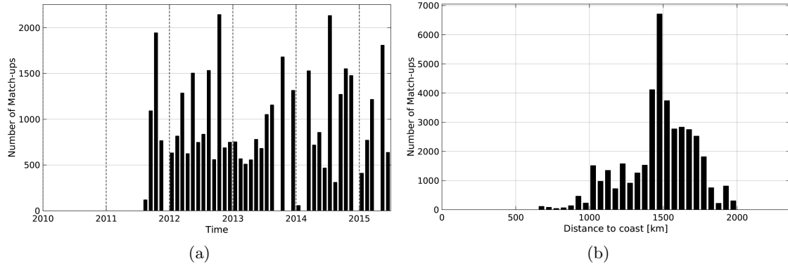
Figure 1: Number of match-ups between TSG-LEGOS-DM and Aquarius-L4-IPRC-V4-WEEKLY SSS as a function of time (a) and as function of the distance to coast (b) over the SPURS 1 Pi-MEP region and for the full satellite product period.
