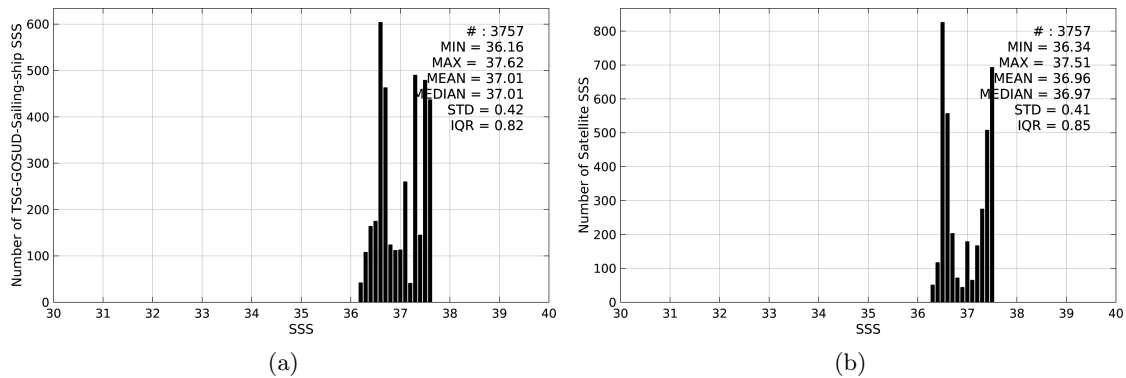
Figure 2: Histograms of SSS from TSG-GOSUD-Sailing-ship (a) and Aquarius-L4-IPRC-V4-WEEKLY (b) considering all match-up pairs per bins of 0.1 over the SPURS 1 Pi-MEP region and for the full satellite product period.
