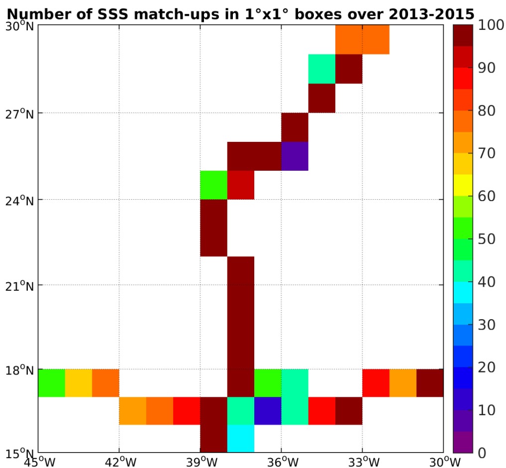
Figure 4: Number of SSS match-ups between TSG-GOSUD-Sailing-ship SSS and the Aquarius-L4-IPRC-V4-WEEKLY SSS product for the SPURS 1 Pi-MEP region over 1°x1° boxes and for the full satellite product period.
