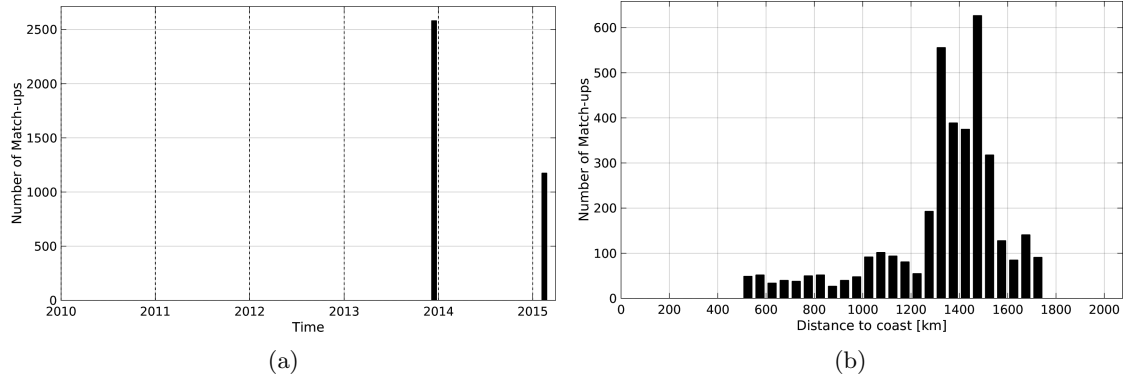
Figure 1: Number of match-ups between TSG-GOSUD-Sailing-ship and Aquarius-L4-IPRC-V4-WEEKLY SSS as a function of time (a) and as function of the distance to coast (b) over the SPURS 1 Pi-MEP region and for the full satellite product period.
