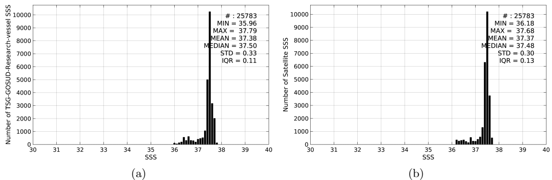
Figure 2: Histograms of SSS from TSG-GOSUD-Research-vessel (a) and Aquarius-L4-IPRC-V4-WEEKLY (b) considering all match-up pairs per bins of 0.1 over the SPURS 1 Pi-MEP region and for the full satellite product period.
