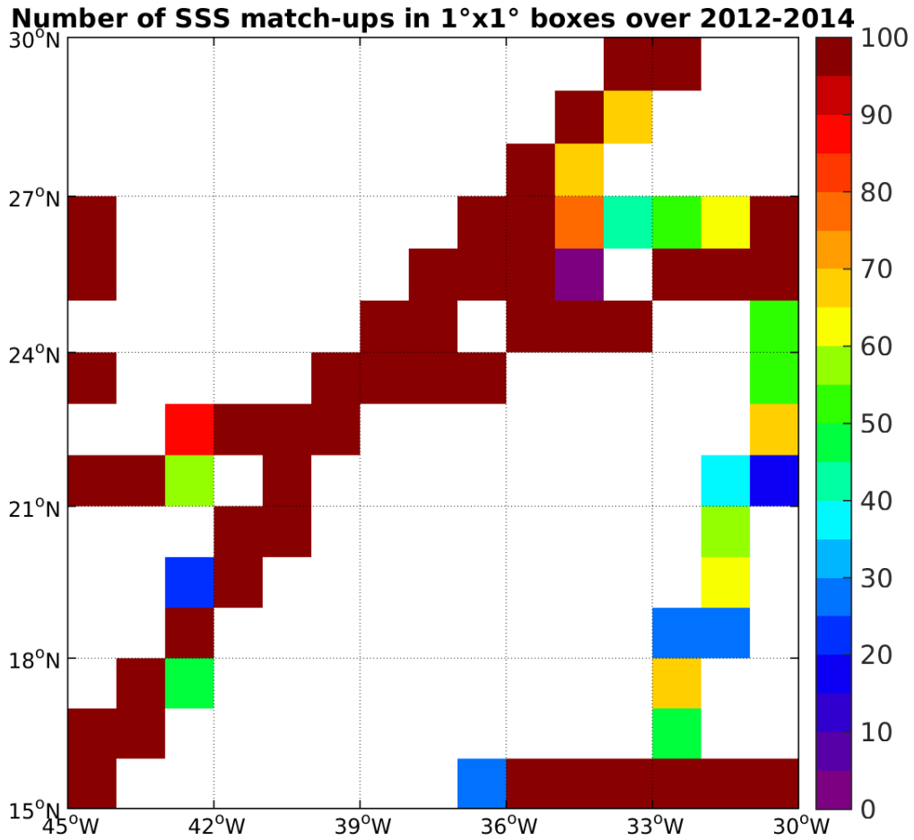
Figure 4: Number of SSS match-ups between TSG-GOSUD-Research-vessel SSS and the Aquarius-L4-IPRC-V4-WEEKLY SSS product for the SPURS 1 Pi-MEP region over 1°x1° boxes and for the full satellite product period.
