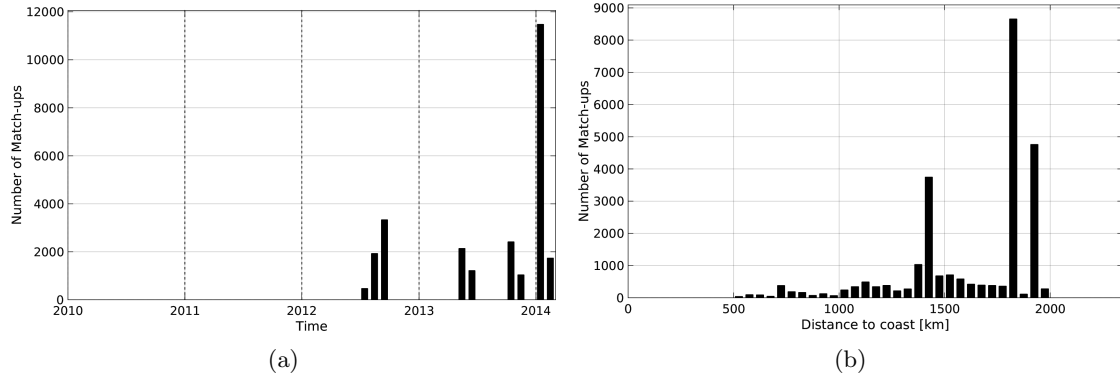
Figure 1: Number of match-ups between TSG-GOSUD-Research-vessel and Aquarius-L4-IPRC-V4-WEEKLY SSS as a function of time (a) and as function of the distance to coast (b) over the SPURS 1 Pi-MEP region and for the full satellite product period.
