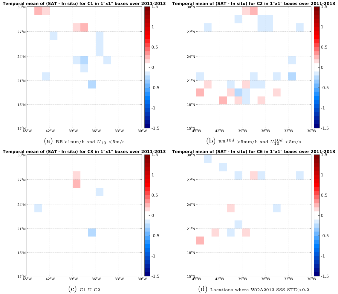
Figure 11: Temporal mean gridded over spatial boxes of size 1°x1° of \Delta SSS (Aquarius-L4-IPRC-V4-WEEKLY - Surface drifters) for 4 different subdatasets corresponding to: RR > 1\text{mm/h} and U_{10} < 5\text{m/s} (a), RR^{10d} > 5\text{mm/h} and U_{10}^{10d} < 5\text{m/s} (b), C1 U C2 (c), Locations where WOA2013 SSS STD > 0.2 (d).
