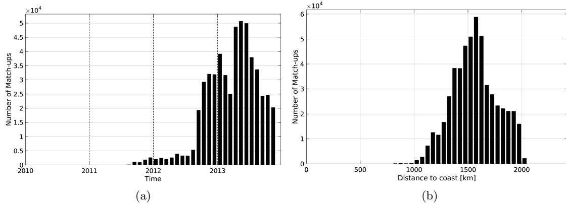
Figure 1: Number of match-ups between Surface drifters and Aquarius-L4-IPRC-V4-WEEKLY SSS as a function of time (a) and as function of the distance to coast (b) over the SPURS 1 Pi-MEP region and for the full satellite product period.
