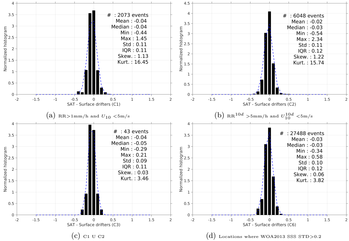
Figure 12: Normalized histogram of \Delta SSS (Aquarius-L4-IPRC-V4-WEEKLY - Surface drifters) for 6 different subdatasets corresponding to: RR > 1mm/h and U_{10} < 5 m/s (a), RR^{10d} > 5 mm/h and U_{10}^{10d} < 5 m/s (b), C1 U C2 (c), Locations where WOA2013 SSS STD > 0.2 (d).
