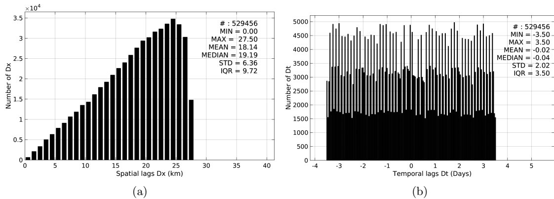
Figure 4: Histograms of the spatial (a) and temporal (b) lags between the time of the Surface drifters measurements and the date of the corresponding Aquarius-L4-IPRC-V4-WEEKLY SSS product.
