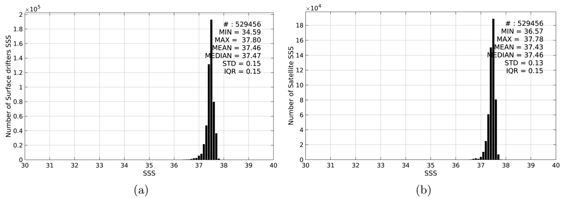
Figure 2: Histograms of SSS from Surface drifters (a) and Aquarius-L4-IPRC-V4-WEEKLY (b) considering all match-up pairs per bins of 0.1 over the SPURS 1 Pi-MEP region and for the full satellite product period.
