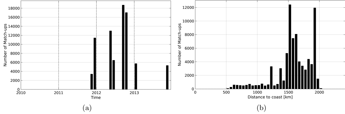
Figure 1: Number of match-ups between TSG-SAMOS and Aquarius-L4-IPRC-V4-MONTHLY SSS as a function of time (a) and as function of the distance to coast (b) over the SPURS 1 Pi-MEP region and for the full satellite product period.
