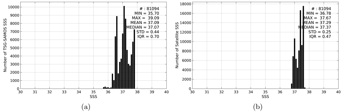
Figure 2: Histograms of SSS from TSG-SAMOS (a) and Aquarius-L4-IPRC-V4-MONTHLY (b) considering all match-up pairs per bins of 0.1 over the SPURS 1 Pi-MEP region and for the full satellite product period.
