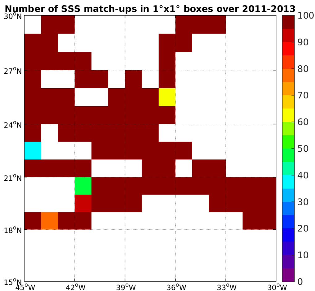
Figure 4: Number of SSS match-ups between TSG-SAMOS SSS and the Aquarius-L4-IPRC-V4-MONTHLY SSS product for the SPURS 1 Pi-MEP region over 1°x1° boxes and for the full satellite product period.
