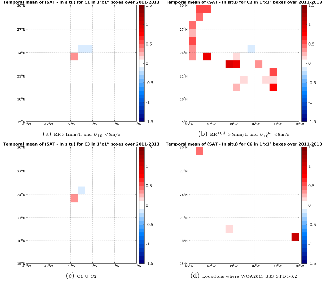
Figure 12: Temporal mean gridded over spatial boxes of size 1^\circ \times 1^\circ of \Delta SSS (Aquarius-L4-IPRC-V4-MONTHLY - TSG-SAMOS) for 4 different subdatasets corresponding to: RR > 1\text{mm/h} and U_{10} < 5\text{m/s} (a), RR^{10d} > 5\text{mm/h} and U_{10}^{10d} < 5\text{m/s} (b), C1 U C2 (c), Locations where WOA2013 SSS STD > 0.2 (d).
