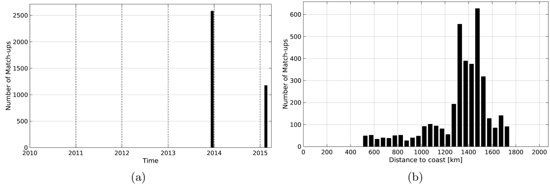
Figure 1: Number of match-ups between TSG-GOSUD-Sailing-ship and Aquarius-L4-IPRC-V4-MONTHLY SSS as a function of time (a) and as function of the distance to coast (b) over the SPURS 1 Pi-MEP region and for the full satellite product period.
