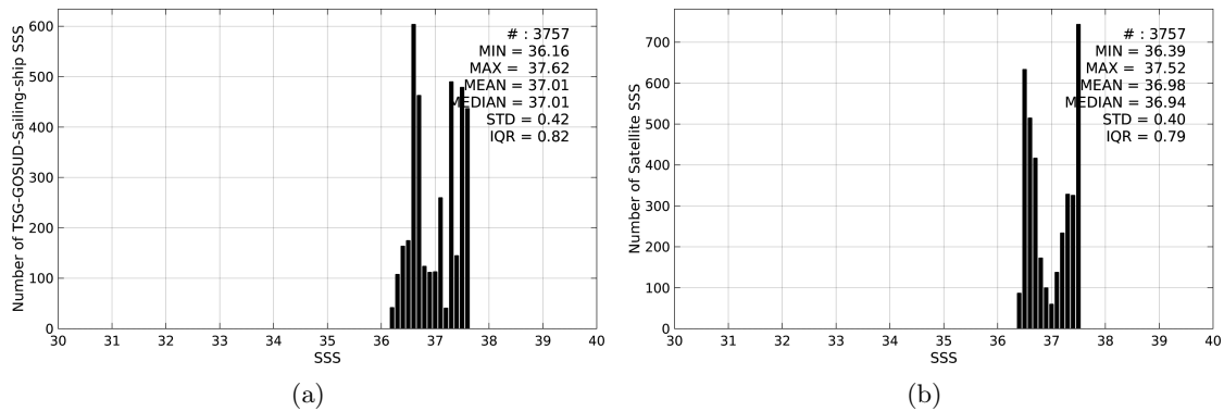
Figure 2: Histograms of SSS from TSG-GOSUD-Sailing-ship (a) and Aquarius-L4-IPRC-V4-MONTHLY (b) considering all match-up pairs per bins of 0.1 over the SPURS 1 Pi-MEP region and for the full satellite product period.
