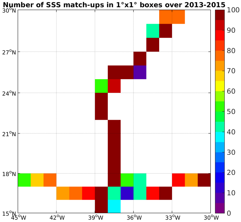
Figure 4: Number of SSS match-ups between TSG-GOSUD-Sailing-ship SSS and the Aquarius-L4-IPRC-V4-MONTHLY SSS product for the SPURS 1 Pi-MEP region over 1°x1° boxes and for the full satellite product period.
