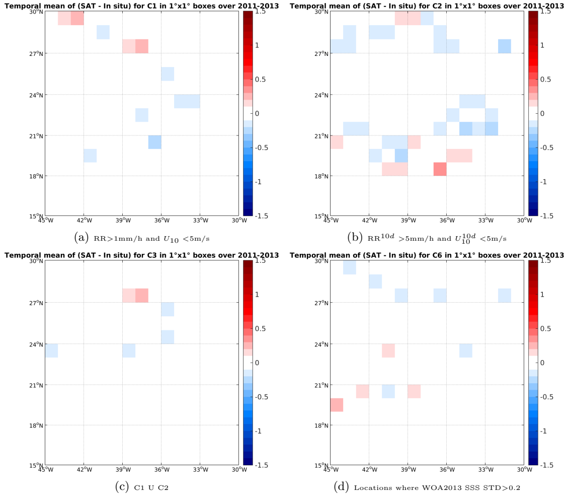
Figure 11: Temporal mean gridded over spatial boxes of size 1°x1° of \Delta SSS (Aquarius-L4-IPRC-V4-MONTHLY - Surface drifters) for 4 different subdatasets corresponding to: RR > 1\text{mm/h} and U_{10} < 5\text{m/s} (a), RR^{10d} > 5\text{mm/h} and U_{10}^{10d} < 5\text{m/s} (b), C1 U C2 (c), Locations where WOA2013 SSS STD > 0.2 (d).
