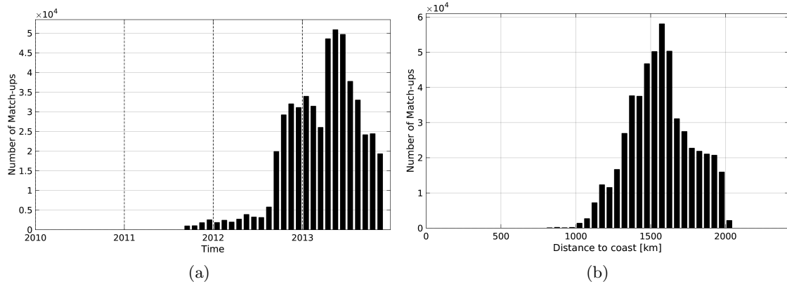
Figure 1: Number of match-ups between Surface drifters and Aquarius-L4-IPRC-V4-MONTHLY SSS as a function of time (a) and as function of the distance to coast (b) over the SPURS 1 Pi-MEP region and for the full satellite product period.
