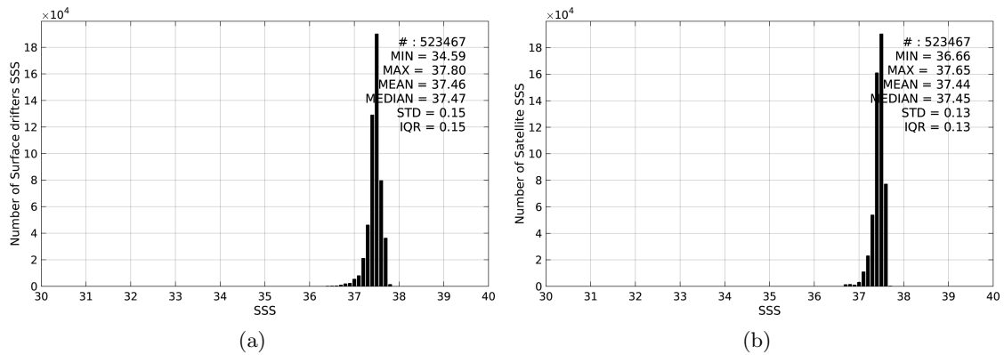
Figure 2: Histograms of SSS from Surface drifters (a) and Aquarius-L4-IPRC-V4-MONTHLY (b) considering all match-up pairs per bins of 0.1 over the SPURS 1 Pi-MEP region and for the full satellite product period.
