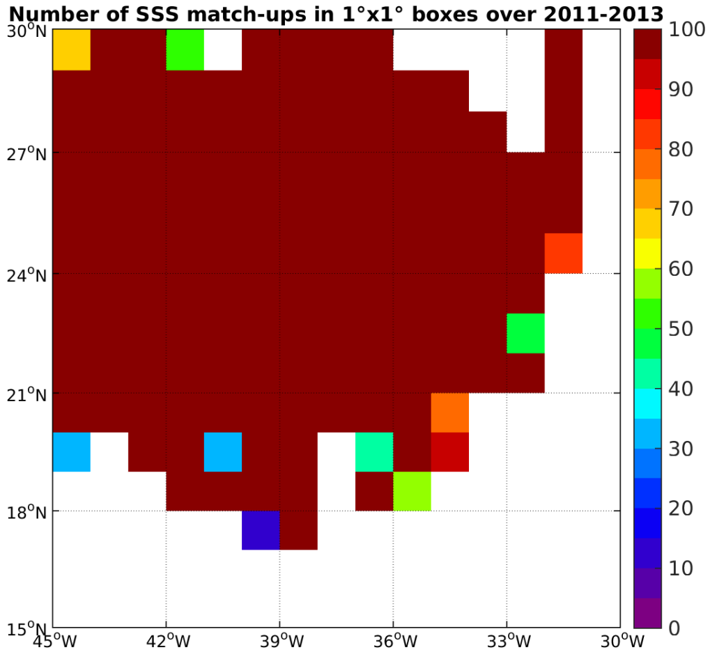
Figure 3: Number of SSS match-ups between Surface drifters SSS and the Aquarius-L4-IPRC-V4-MONTHLY SSS product for the SPURS 1 Pi-MEP region over 1°x1° boxes and for the full satellite product period.
