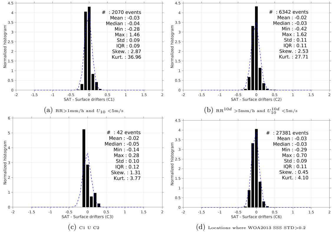
Figure 12: Normalized histogram of \Delta SSS (Aquarius-L4-IPRC-V4-MONTHLY - Surface drifters) for 6 different subdatasets corresponding to: RR > 1\text{mm/h} and U_{10} < 5\text{m/s} (a), RR^{10d} > 5\text{mm/h} and U_{10}^{10d} < 5\text{m/s} (b), C1 U C2 (c), Locations where WOA2013 SSS STD > 0.2 (d).
