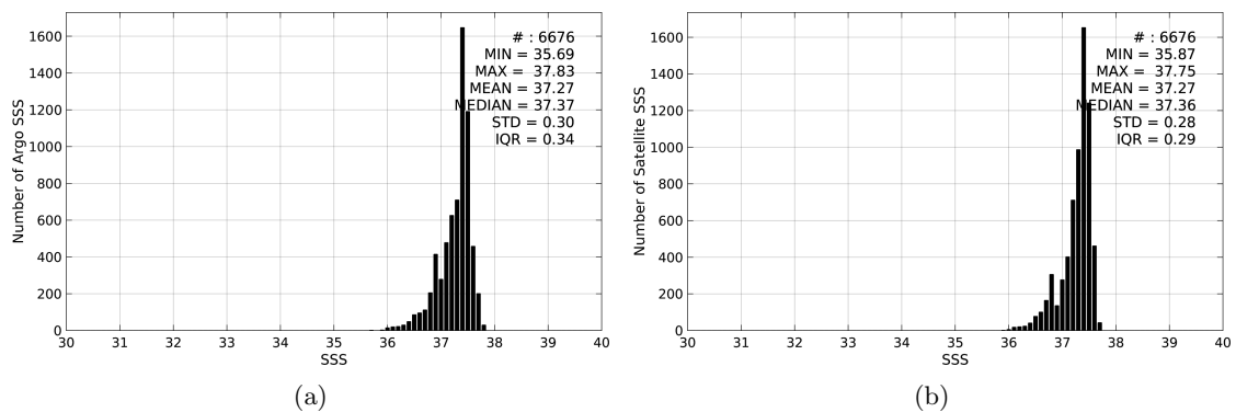
Figure 2: Histograms of SSS from Argo (a) and Aquarius-L4-IPRC-V4-MONTHLY (b) considering all match-up pairs per bins of 0.1 over the SPURS 1 Pi-MEP region and for the full satellite product period.
