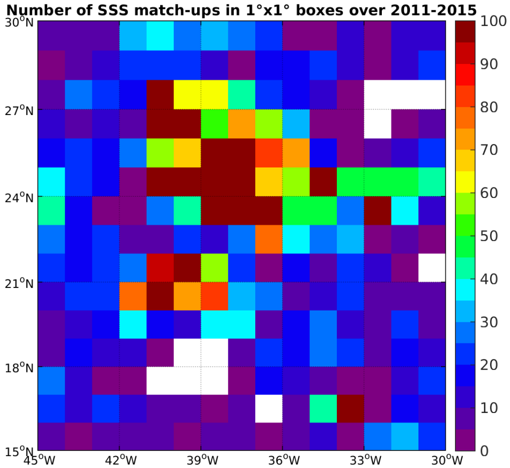
Figure 4: Number of SSS match-ups between Argo SSS and the Aquarius-L4-IPRC-V4-MONTHLY SSS product for the SPURS 1 Pi-MEP region over 1°x1° boxes and for the full satellite product period.
