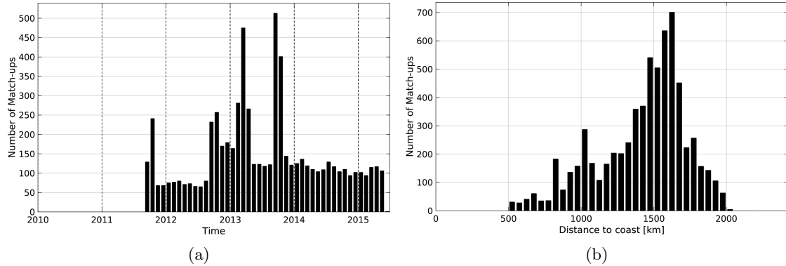
Figure 1: Number of match-ups between Argo and Aquarius-L4-IPRC-V4-MONTHLY SSS as a function of time (a) and as function of the distance to coast (b) over the SPURS 1 Pi-MEP region and for the full satellite product period.
