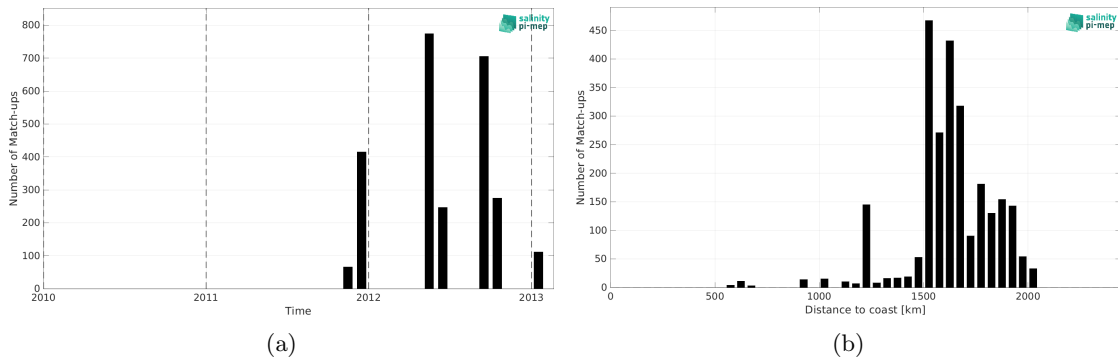
Figure 2: Number of match-ups between TSG (SAMOS) and Aquarius SSS L3 OR v5 - 7-Day running (NASA-GSFC) SSS as a function of time (a) and as function of the distance to coast (b) over the SPURS 1 Pi-MEP region and for the full satellite product period.
