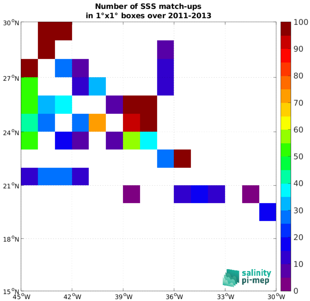
Figure 5: Number of SSS match-ups between TSG (SAMOS) SSS and the Aquarius SSS L3 OR v5 - 7-Day running (NASA-GSFC) SSS product for the SPURS 1 Pi-MEP region over 1°x1° boxes and for the full satellite product period.
