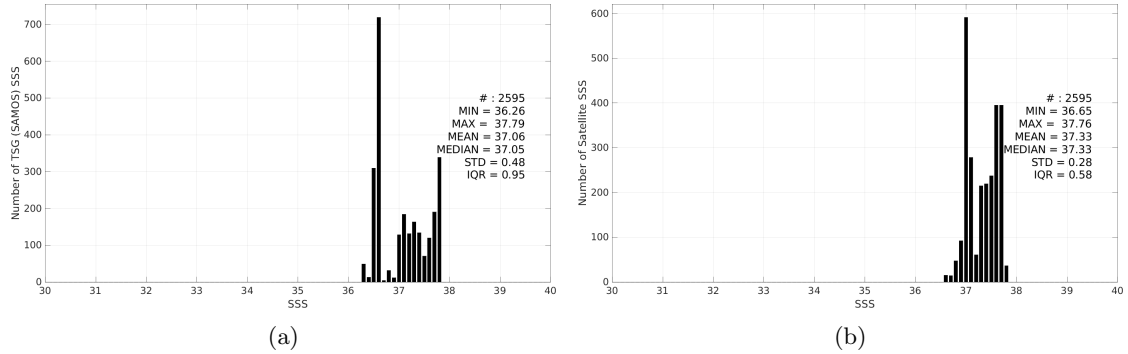
Figure 3: Histograms of SSS from TSG (SAMOS) (a) and Aquarius SSS L3 OR v5 - 7-Day running (NASA-GSFC) (b) considering all match-up pairs per bins of 0.1 over the SPURS 1 Pi-MEP region and for the full satellite product period.
