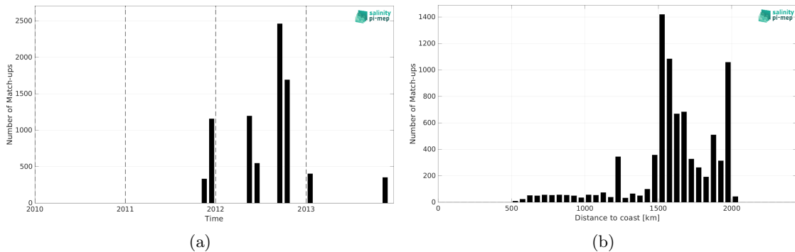
Figure 1: Number of match-ups between TSG (SAMOS) and Aquarius SSS L3 OR v5 - 7-Day running (NASA-GSFC) SSS as a function of time (a) and as function of the distance to coast (b) over the SPURS 1 Pi-MEP region and for the full satellite product period.
