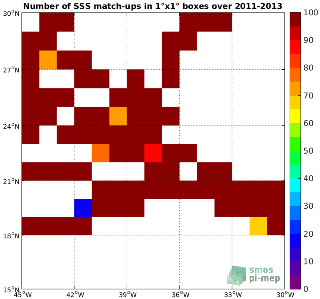
Figure 4: Number of SSS match-ups between TSG-SAMOS SSS and the Aquarius-L3-OR-V5-7DAY-RUNNING-1DEG SSS product for the SPURS 1 Pi-MEP region over 1°x1° boxes and for the full satellite product period.
