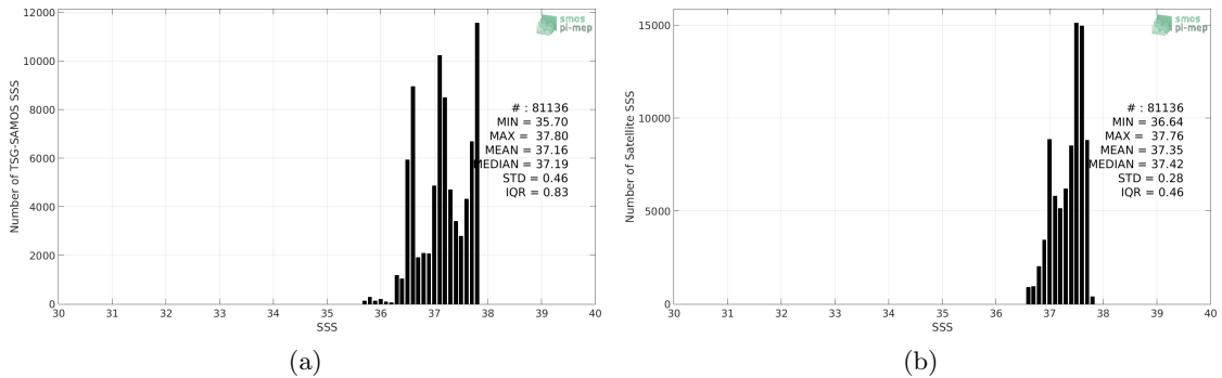
Figure 2: Histograms of SSS from TSG-SAMOS (a) and Aquarius-L3-OR-V5-7DAY-RUNNING-1DEG (b) considering all match-up pairs per bins of 0.1 over the SPURS 1 Pi-MEP region and for the full satellite product period.
