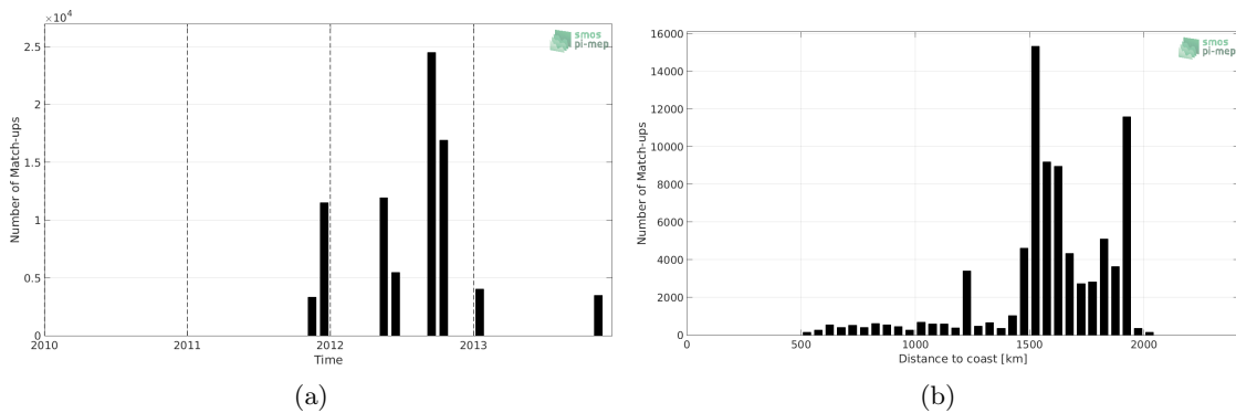
Figure 1: Number of match-ups between TSG-SAMOS and Aquarius-L3-OR-V5-7DAY-RUNNING-1DEG SSS as a function of time (a) and as function of the distance to coast (b) over the SPURS 1 Pi-MEP region and for the full satellite product period.
