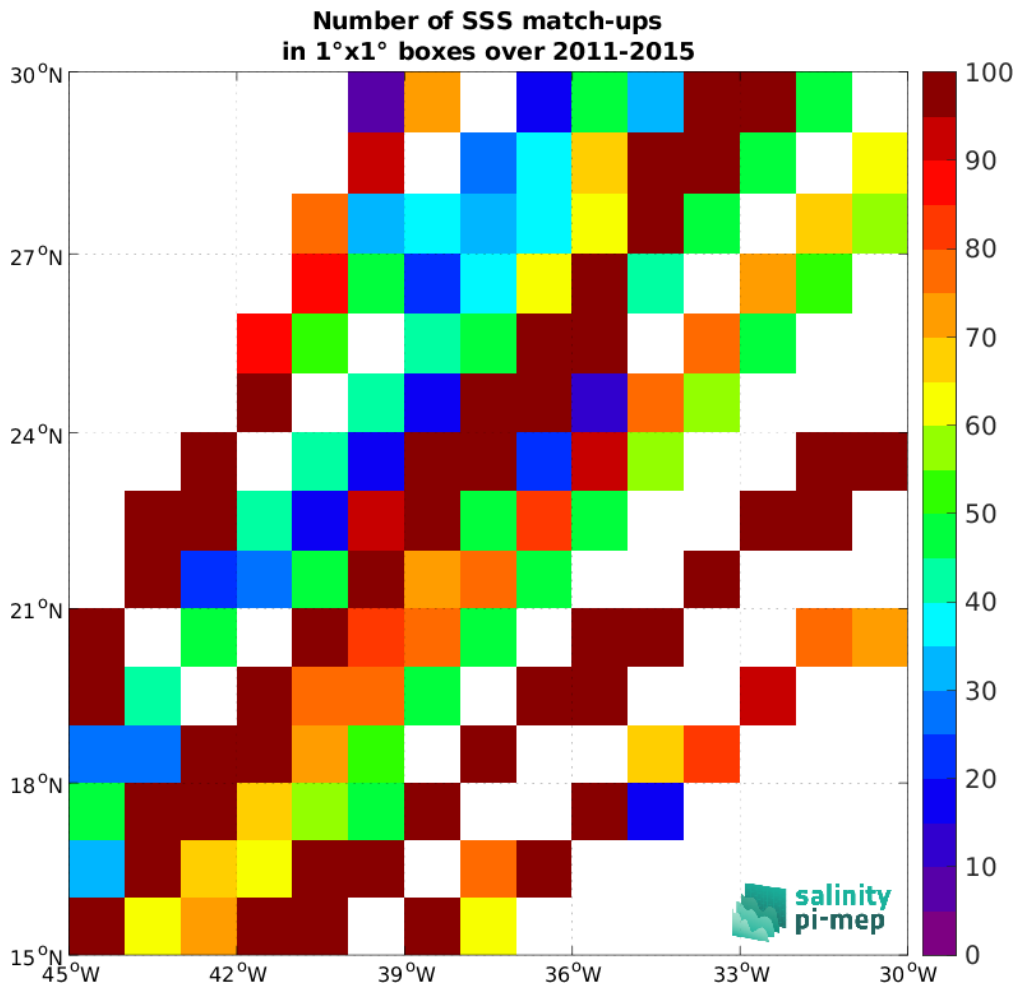
Figure 4: Number of SSS match-ups between TSG (LEGOS-DM) SSS and the Aquarius SSS L3 OR v5 - 7-Day running (NASA-GSFC) SSS product for the SPURS 1 Pi-MEP region over 1°x1° boxes and for the full satellite product period.
