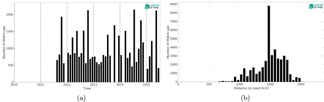
Figure 1: Number of match-ups between TSG (LEGOS-DM) and Aquarius SSS L3 OR v5 - 7-Day running (NASA-GSFC) SSS as a function of time (a) and as function of the distance to coast (b) over the SPURS 1 Pi-MEP region and for the full satellite product period.
