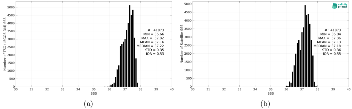
Figure 2: Histograms of SSS from TSG (LEGOS-DM) (a) and Aquarius SSS L3 OR v5 - 7-Day running (NASA-GSFC) (b) considering all match-up pairs per bins of 0.1 over the SPURS 1 Pi-MEP region and for the full satellite product period.
