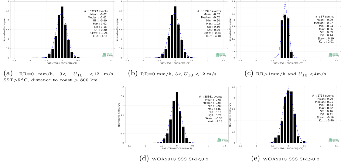
Figure 13: Normalized histogram of \Delta\text{SSS} (Aquarius SSS L3 OR v5 - 7-Day running (NASA-GSFC) - TSG (LEGOS-DM)) for 5 different subdatasets corresponding to: RR=0 mm/h, 3 < U_{10} < 12 m/s, SST > 5°C, distance to coast > 800 km (a), RR=0 mm/h, 3 < U_{10} < 12 m/s (b), RR > 1mm/h and U_{10} < 4 m/s (c), WOA2013 SSS Std < 0.2 (d), WOA2013 SSS Std > 0.2 (e).
