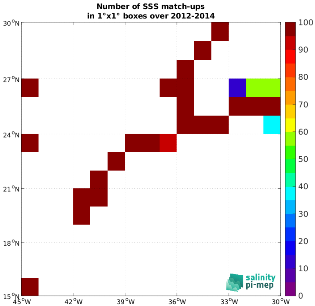
Figure 5: Number of SSS match-ups between TSG (GOSUD-Research-vessel) SSS and the Aquarius SSS L3 OR v5 - 7-Day running (NASA-GSFC) SSS product for the SPURS 1 Pi-MEP region over 1^\circ \times 1^\circ boxes and for the full satellite product period.
