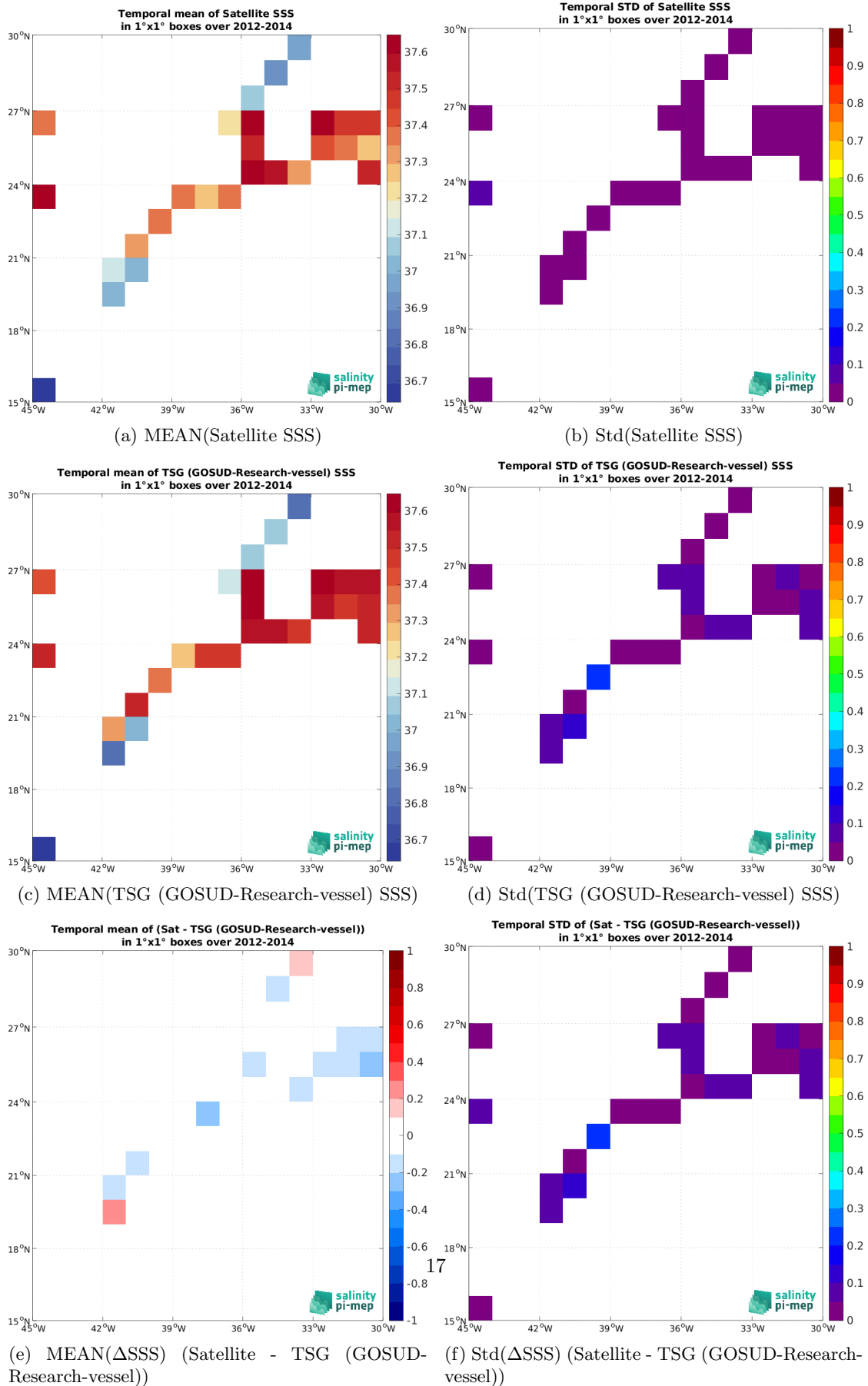
Figure 7: Temporal mean (left) and Std (right) of SSS from Aquarius SSS L3 OR v5 - 7-Day running (NASA-GSFC) (top), TSG (GOSUD-Research-vessel) (middle), and of \Delta SSS (Satellite - TSG (GOSUD-Research-vessel)). Only match-up pairs are used to generate these maps.
