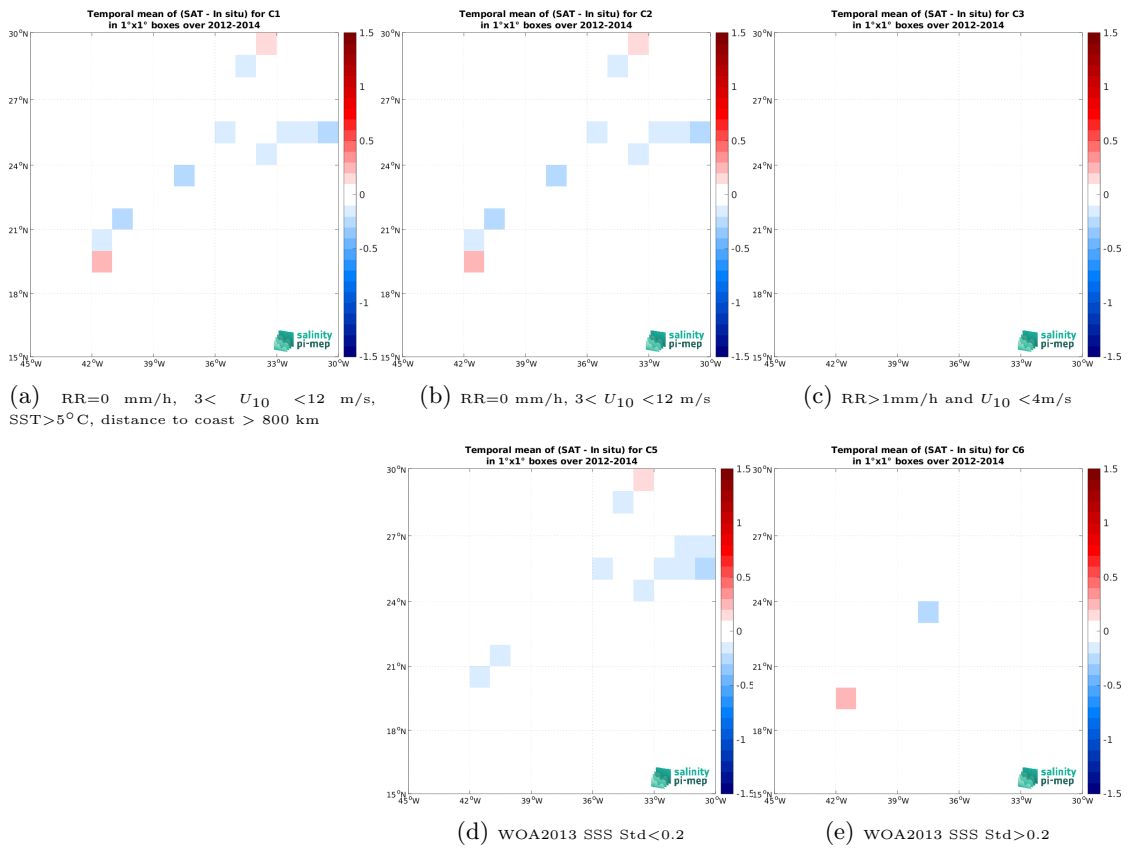
Figure 14: Temporal mean gridded over spatial boxes of size 1^\circ \times 1^\circ of \Delta SSS (Aquarius SSS L3 OR v5 - 7-Day running (NASA-GSFC) - TSG (GOSUD-Research-vessel)) for 5 different subdatasets corresponding to: RR=0 mm/h, 3 < U_{10} < 12 m/s, SST > 5^\circ C , distance to coast > 800 km (a), RR=0 mm/h, 3 < U_{10} < 12 m/s (b), RR > 1 mm/h and U_{10} < 4 m/s (c), WOA2013 SSS Std <0.2 (d), WOA2013 SSS Std >0.2 (e).
