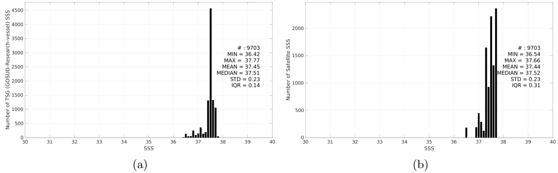
Figure 3: Histograms of SSS from TSG (GOSUD-Research-vessel) (a) and Aquarius SSS L3 OR v5 - 7-Day running (NASA-GSFC) (b) considering all match-up pairs per bins of 0.1 over the SPURS 1 Pi-MEP region and for the full satellite product period.
