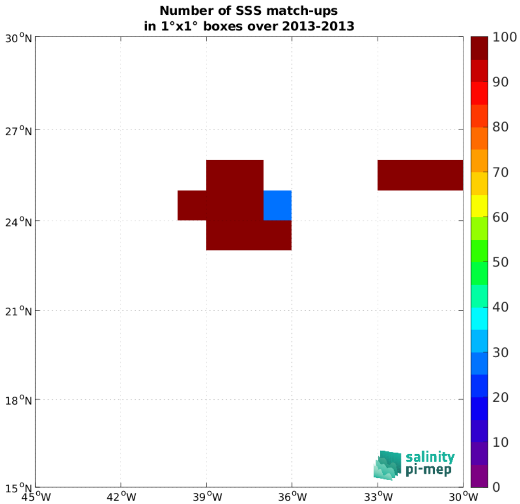
Figure 5: Number of SSS match-ups between TSG (CSIC-UTM) SSS and the Aquarius SSS L3 OR v5 - 7-Day running (NASA-GSFC) SSS product for the SPURS 1 Pi-MEP region over 1°x1° boxes and for the full satellite product period.
