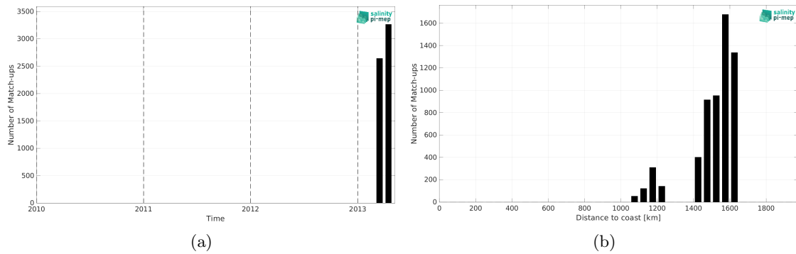
Figure 2: Number of match-ups between TSG (CSIC-UTM) and Aquarius SSS L3 OR v5 - 7-Day running (NASA-GSFC) SSS as a function of time (a) and as function of the distance to coast (b) over the SPURS 1 Pi-MEP region and for the full satellite product period.
