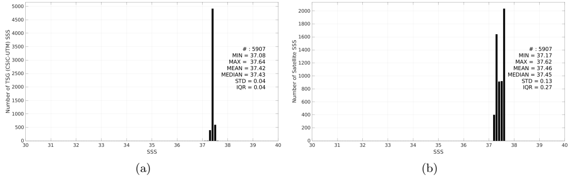
Figure 3: Histograms of SSS from TSG (CSIC-UTM) (a) and Aquarius SSS L3 OR v5 - 7-Day running (NASA-GSFC) (b) considering all match-up pairs per bins of 0.1 over the SPURS 1 Pi-MEP region and for the full satellite product period.
