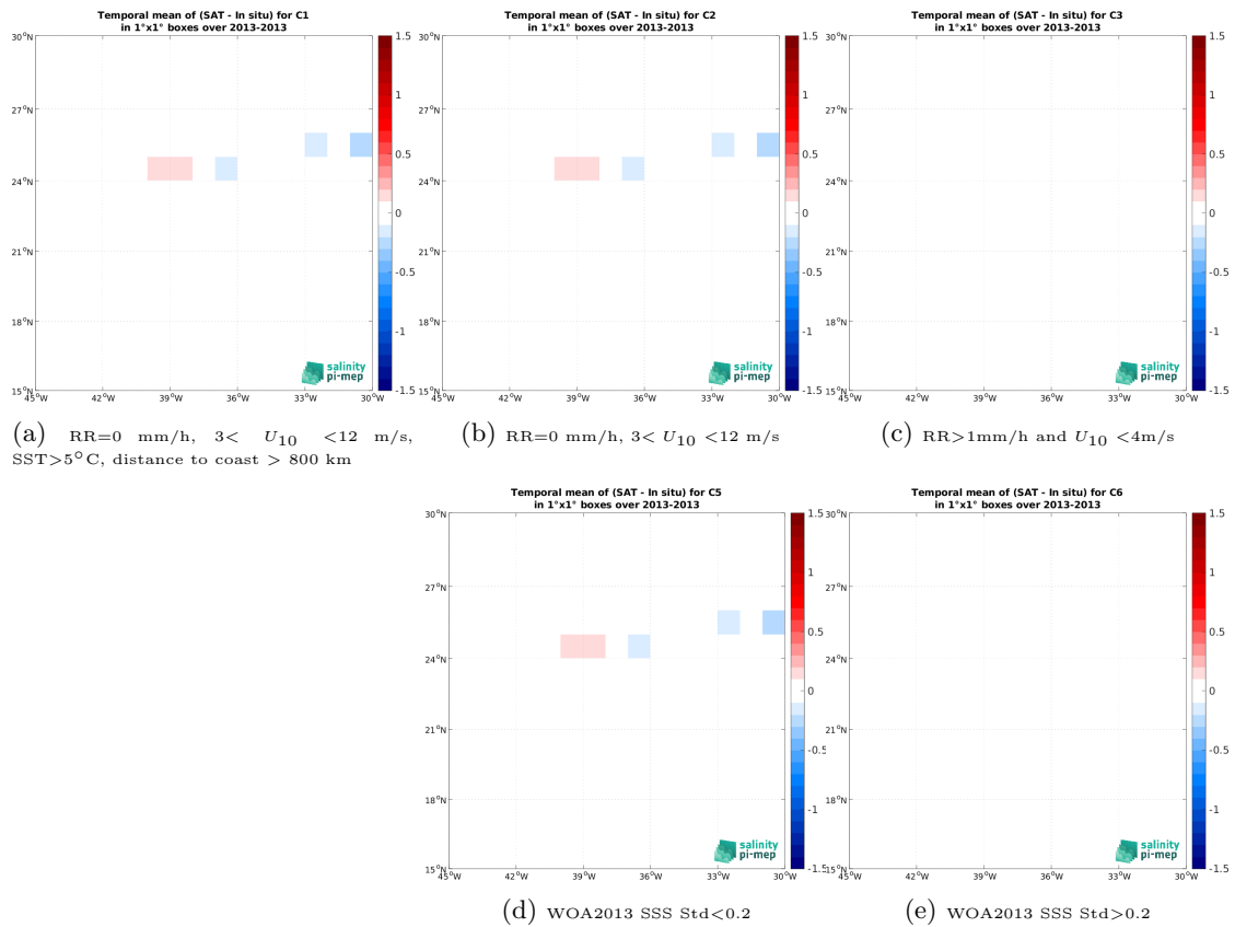
Figure 14: Temporal mean gridded over spatial boxes of size 1^\circ \times 1^\circ of \Delta SSS (Aquarius SSS L3 OR v5 - 7-Day running (NASA-GSFC) - TSG (CSIC-UTM)) for 5 different subdatasets corresponding to: RR=0 mm/h, 3 < U_{10} < 12 m/s, SST > 5^\circ C , distance to coast > 800 km (a), RR=0 mm/h, 3 < U_{10} < 12 m/s (b), RR > 1 mm/h and U_{10} < 4 m/s (c), WOA2013 SSS Std < 0.2 (d), WOA2013 SSS Std > 0.2 (e).
