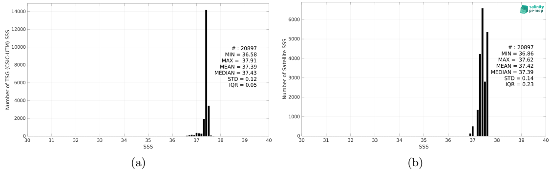
Figure 2: Histograms of SSS from TSG (CSIC-UTM) (a) and Aquarius SSS L3 OR v5 - 7-Day running (NASA-GSFC) (b) considering all match-up pairs per bins of 0.1 over the SPURS 1 Pi-MEP region and for the full satellite product period.
