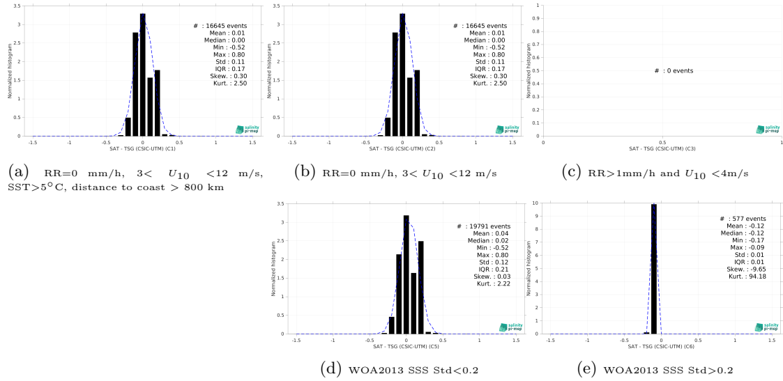
Figure 13: Normalized histogram of \Delta SSS (Aquarius SSS L3 OR v5 - 7-Day running (NASA-GSFC) - TSG (CSIC-UTM)) for 5 different subdatasets corresponding to: RR=0 mm/h, 3 < U_{10} < 12 m/s, SST > 5°C, distance to coast > 800 km (a), RR=0 mm/h, 3 < U_{10} < 12 m/s (b), RR > 1mm/h and U_{10} < 4 m/s (c), WOA2013 SSS Std < 0.2 (d), WOA2013 SSS Std > 0.2 (e).
