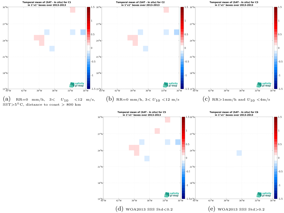
Figure 12: Temporal mean gridded over spatial boxes of size 1^{\circ}\times 1^{\circ} of \Delta\text{SSS} (Aquarius SSS L3 OR v5 - 7-Day running (NASA-GSFC) - TSG (CSIC-UTM)) for 5 different subdatasets corresponding to:RR=0 mm/h, 3 < U_{10} < 12 m/s, SST >5^{\circ}\text{C} , distance to coast > 800 km (a), RR=0 mm/h, 3 < U_{10} < 12 m/s (b), RR >1 mm/h and U_{10} < 4 m/s (c), WOA2013 SSS Std <0.2 (d), WOA2013 SSS Std >0.2 (e).
