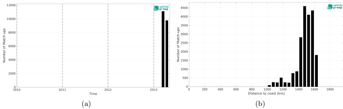
Figure 1: Number of match-ups between TSG (CSIC-UTM) and Aquarius SSS L3 OR v5 - 7-Day running (NASA-GSFC) SSS as a function of time (a) and as function of the distance to coast (b) over the SPURS 1 Pi-MEP region and for the full satellite product period.
