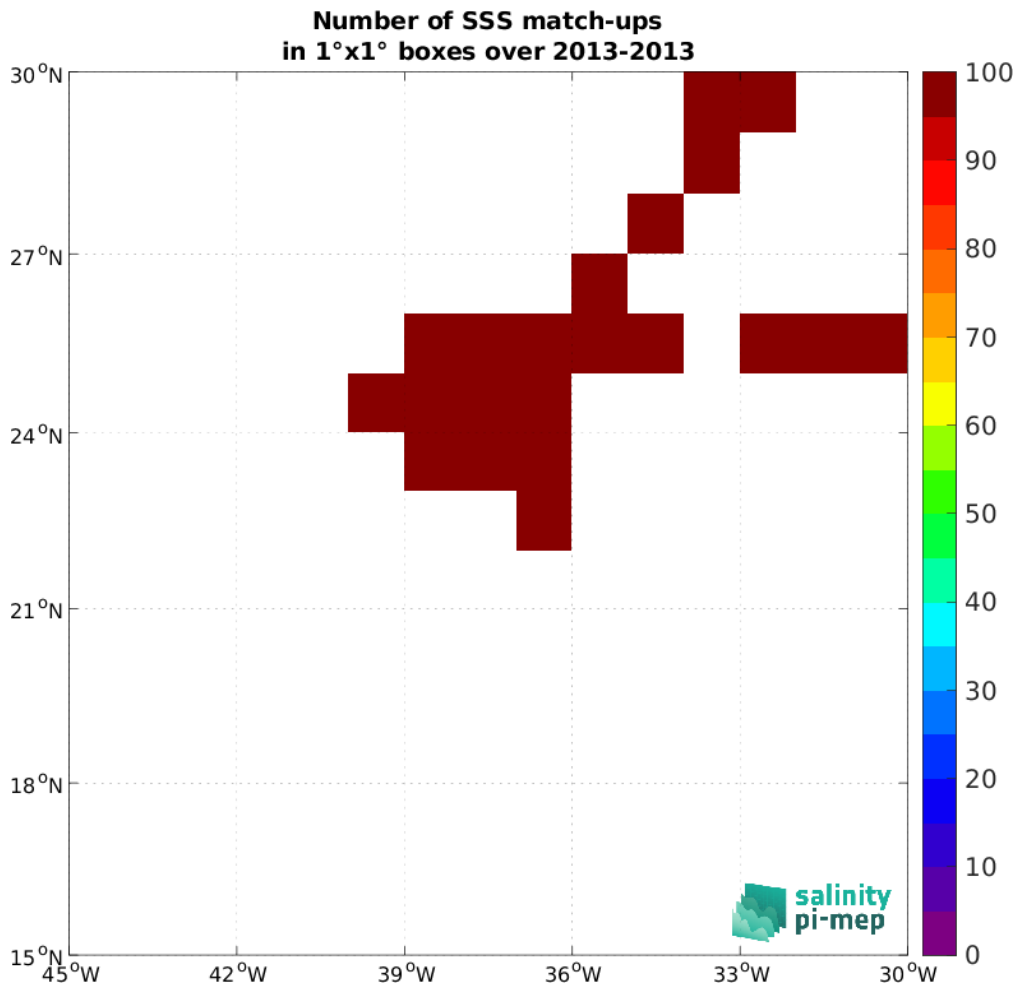
Figure 4: Number of SSS match-ups between TSG (CSIC-UTM) SSS and the Aquarius SSS L3 OR v5 - 7-Day running (NASA-GSFC) SSS product for the SPURS 1 Pi-MEP region over 1°x1° boxes and for the full satellite product period.
