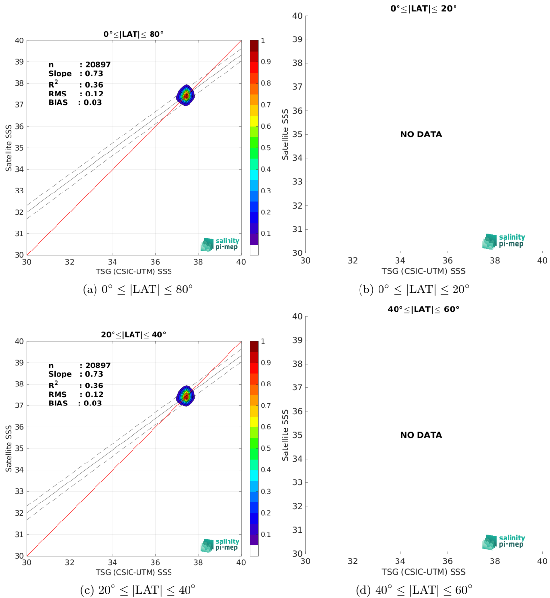
Figure 9: Contour maps of the concentration of Aquarius SSS L3 OR v5 - 7-Day running (NASA-GSFC) SSS (y-axis) versus TSG (CSIC-UTM) SSS (x-axis) at match-up pairs for different latitude bands. For each plot, the red line shows x=y . The black thin and dashed lines indicate a linear fit through the data cloud and the \pm 95\% confidence levels, respectively. The number match-up pairs n , the slope and R^2 coefficient of the linear fit, the root mean square (RMS) and the mean bias between satellite and in situ data are indicated for each latitude band in each plots.
