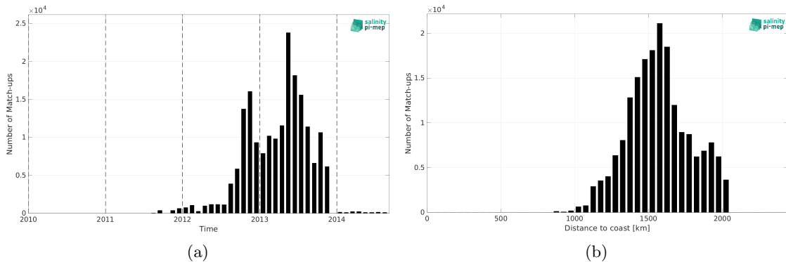
Figure 2: Number of match-ups between Surface drifters and Aquarius SSS L3 OR v5 - 7-Day running (NASA-GSFC) SSS as a function of time (a) and as function of the distance to coast (b) over the SPURS 1 Pi-MEP region and for the full satellite product period.
