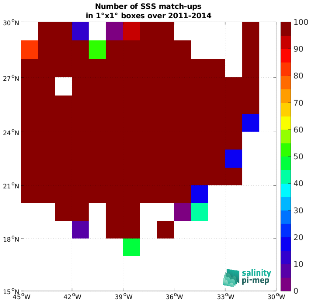
Figure 4: Number of SSS match-ups between Surface drifters SSS and the Aquarius SSS L3 OR v5 - 7-Day running (NASA-GSFC) SSS product for the SPURS 1 Pi-MEP region over 1°x1° boxes and for the full satellite product period.
