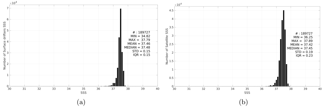
Figure 3: Histograms of SSS from Surface drifters (a) and Aquarius SSS L3 OR v5 - 7-Day running (NASA-GSFC) (b) considering all match-up pairs per bins of 0.1 over the SPURS 1 Pi-MEP region and for the full satellite product period.
